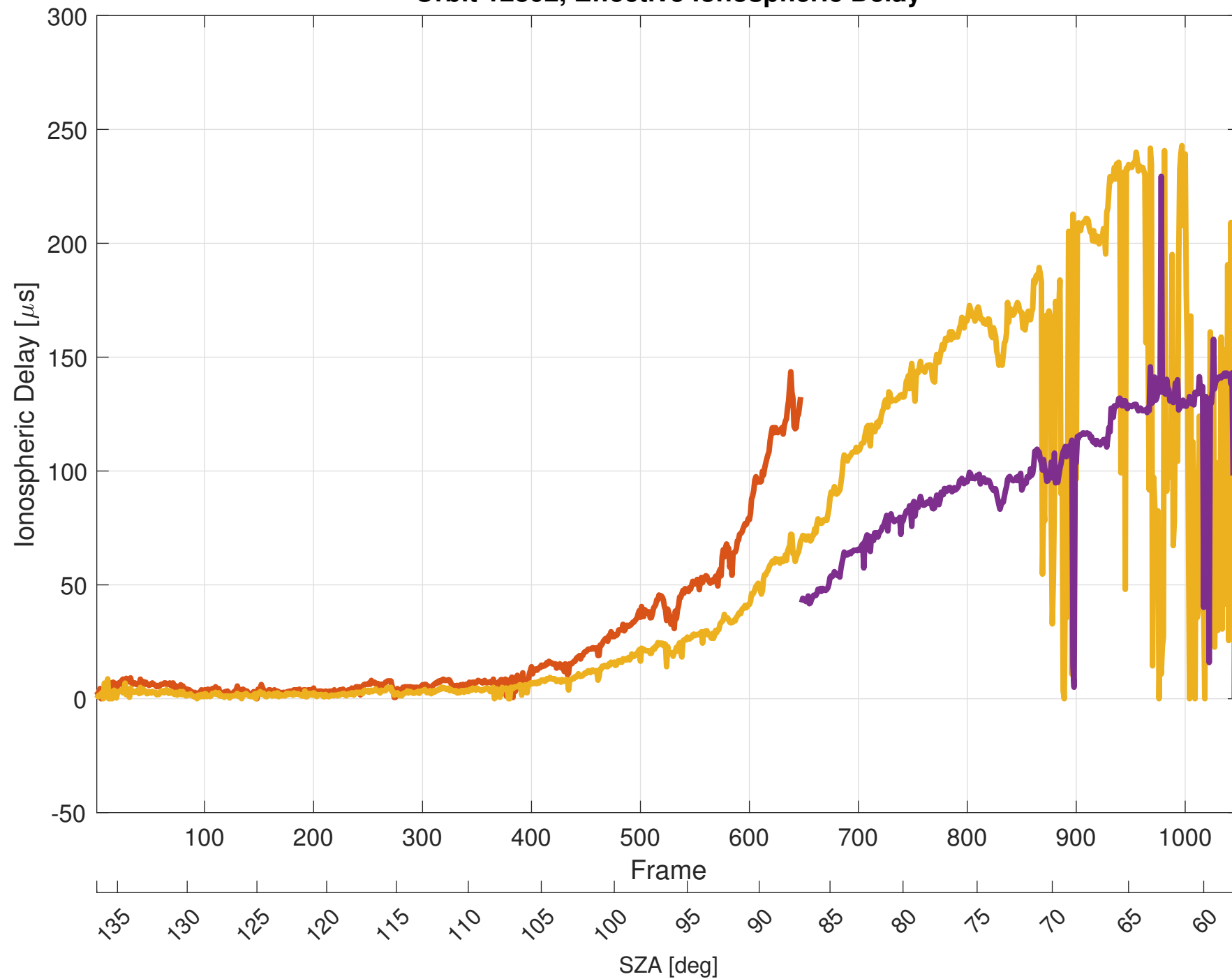
Orbit 12802, Effective Ionospheric Delay
