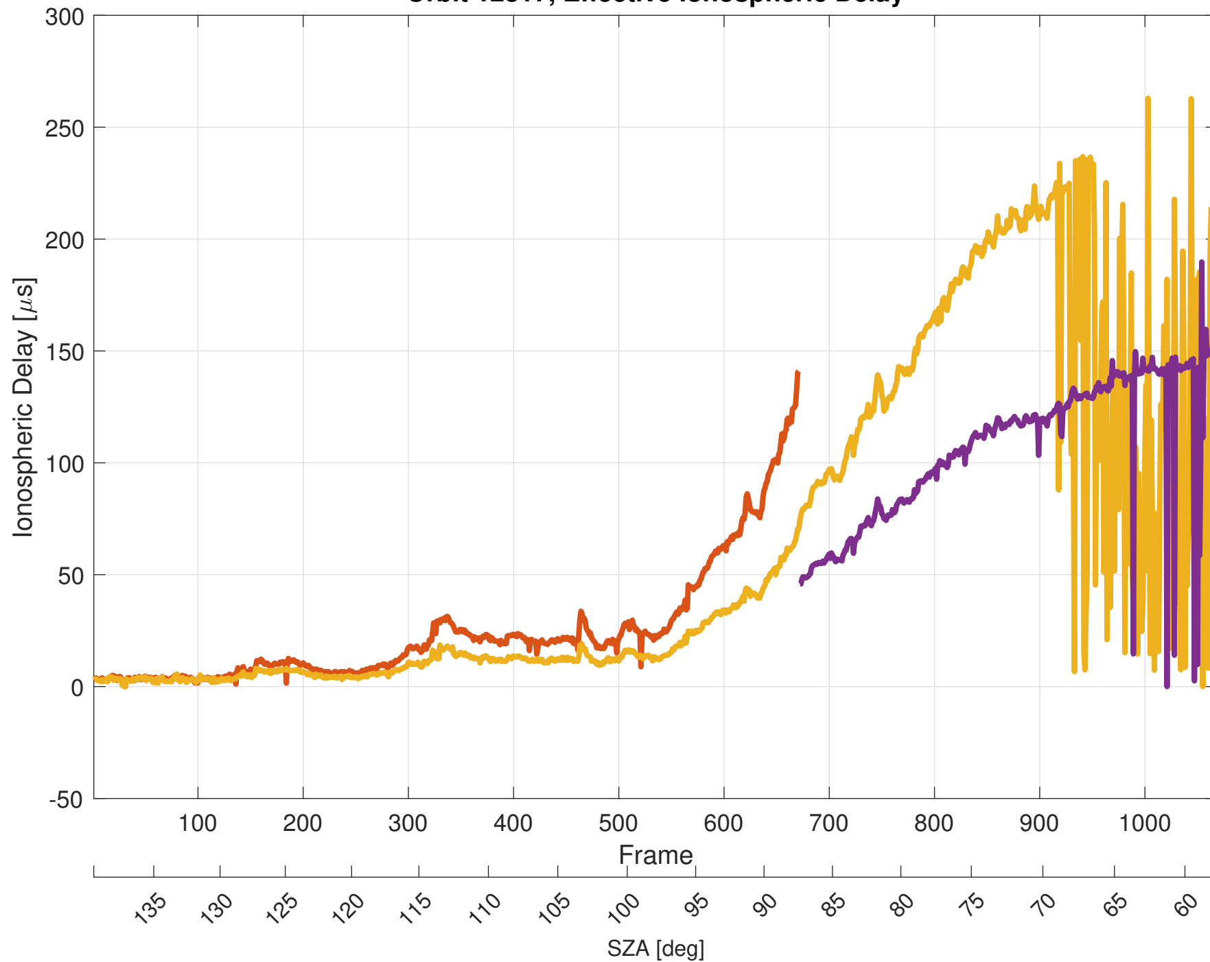
Orbit 12817, Effective Ionospheric Delay
