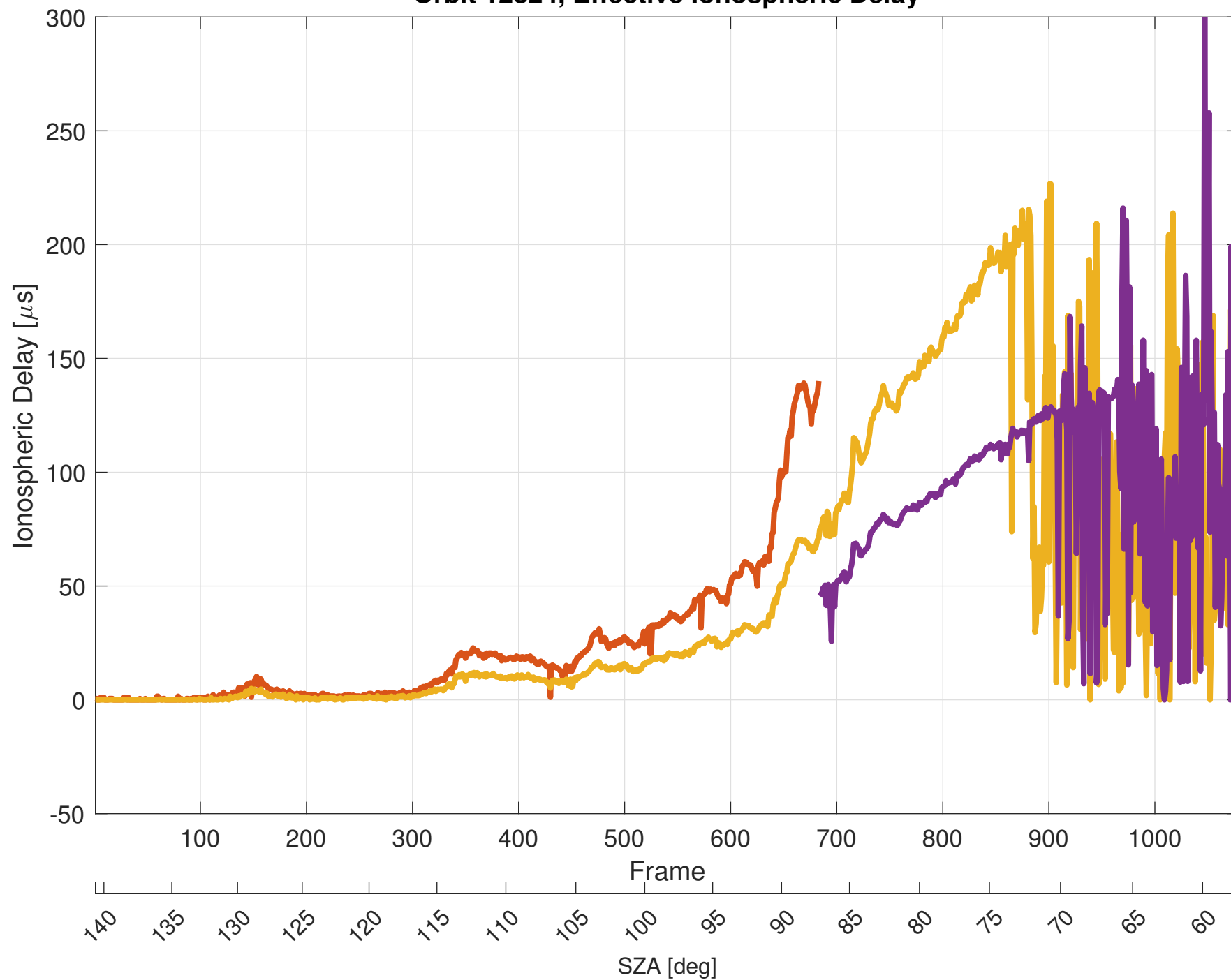
Orbit 12824, Effective Ionospheric Delay
