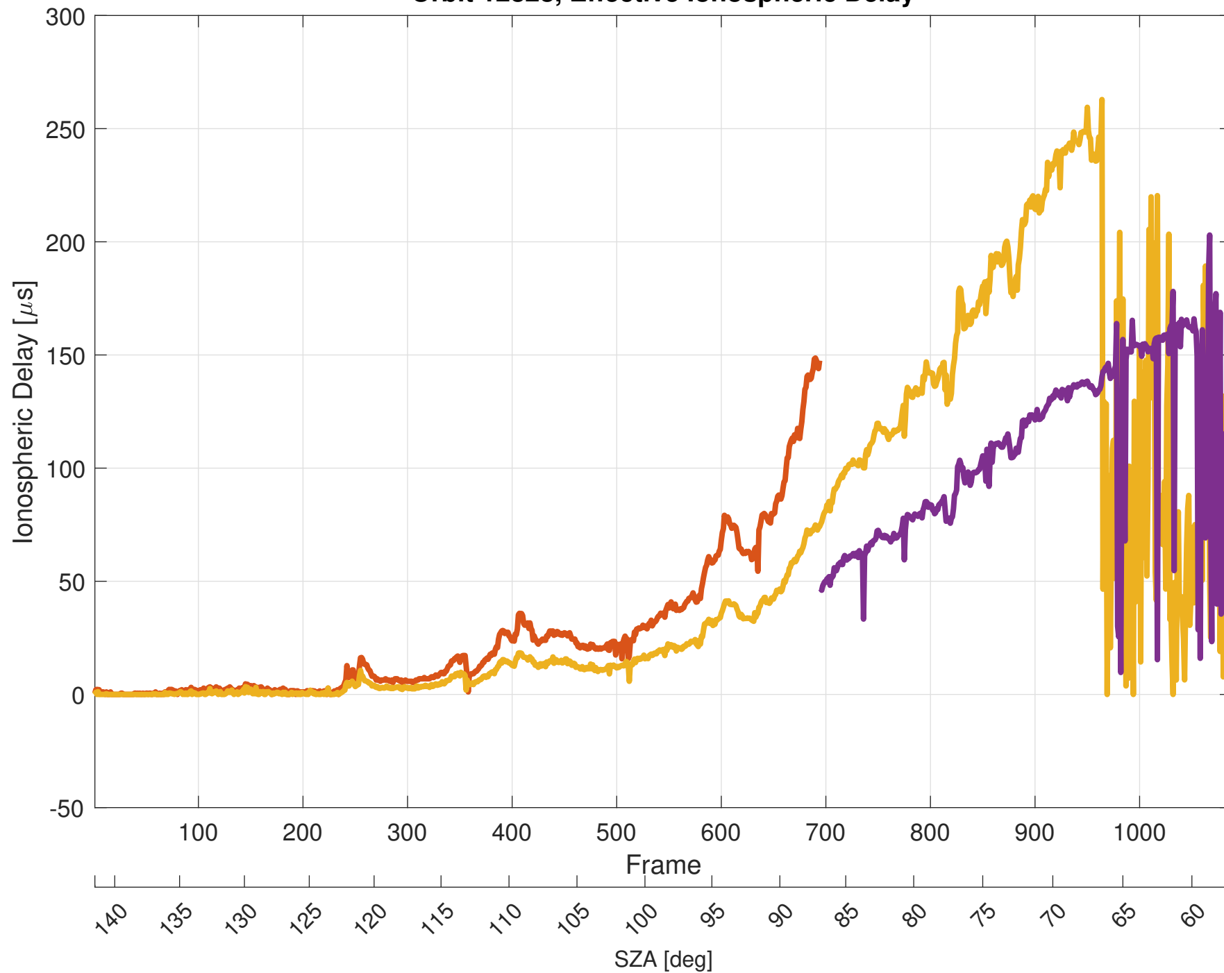
Orbit 12828, Effective Ionospheric Delay
