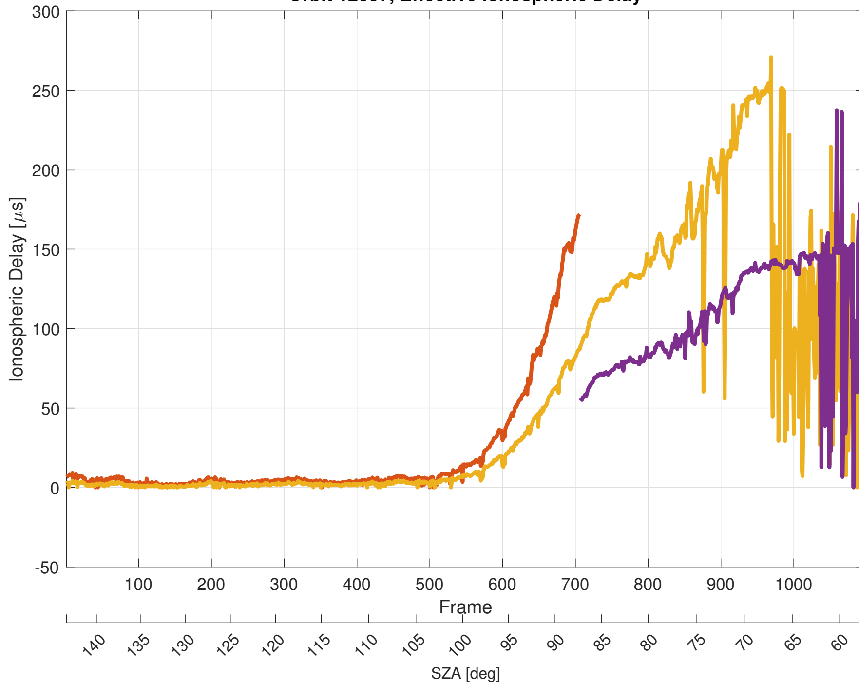
Orbit 12837, Effective Ionospheric Delay
