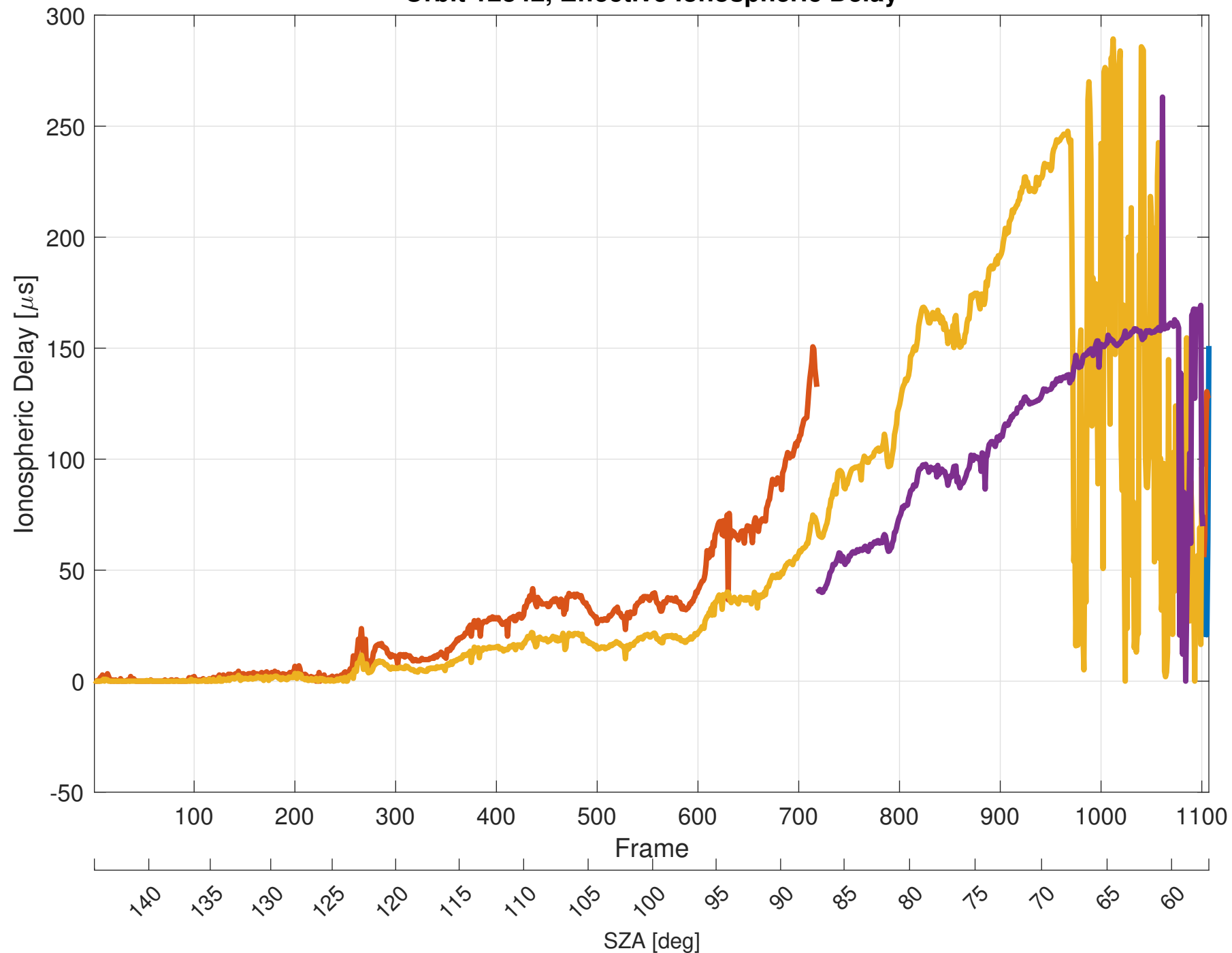
Orbit 12842, Effective Ionospheric Delay
