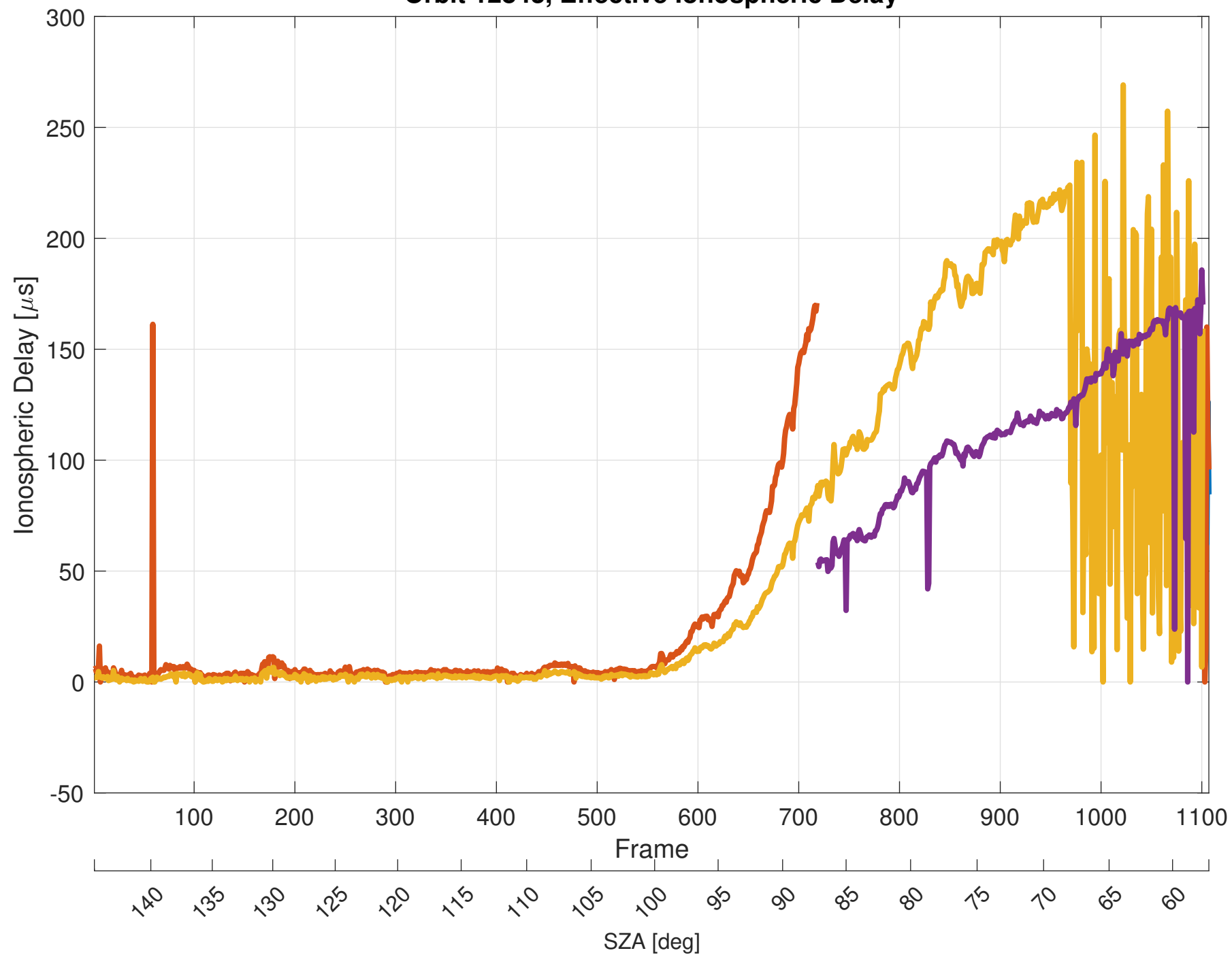
Orbit 12843, Effective Ionospheric Delay
