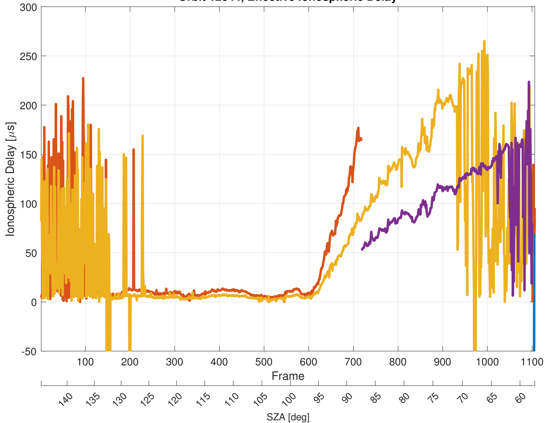
Orbit 12844, Effective Ionospheric Delay
