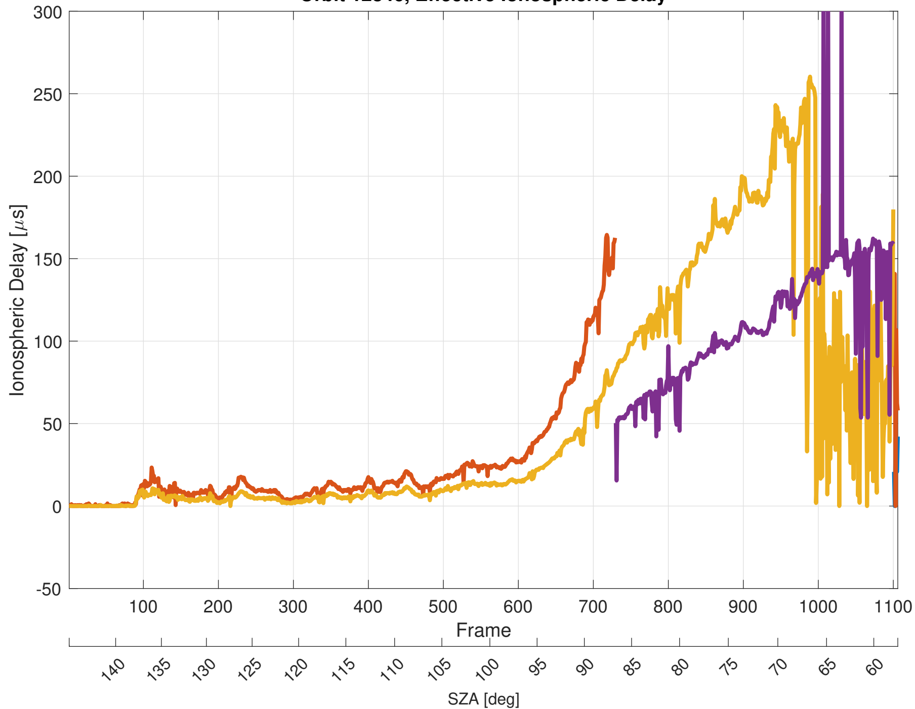
Orbit 12846, Effective Ionospheric Delay
