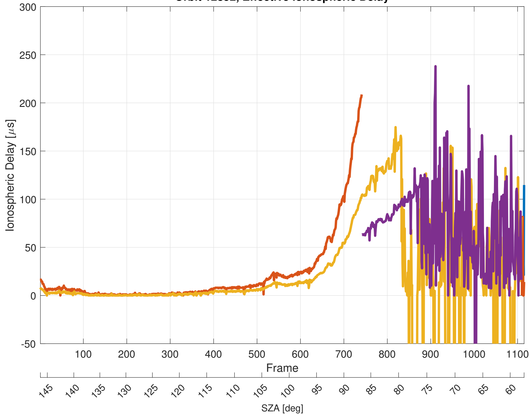
Orbit 12852, Effective Ionospheric Delay
