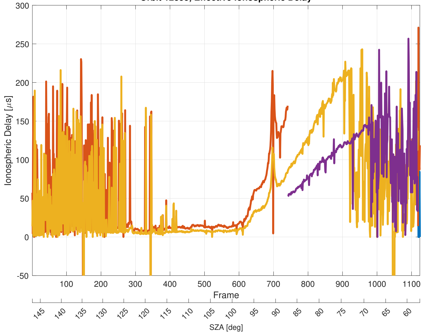
Orbit 12855, Effective Ionospheric Delay
