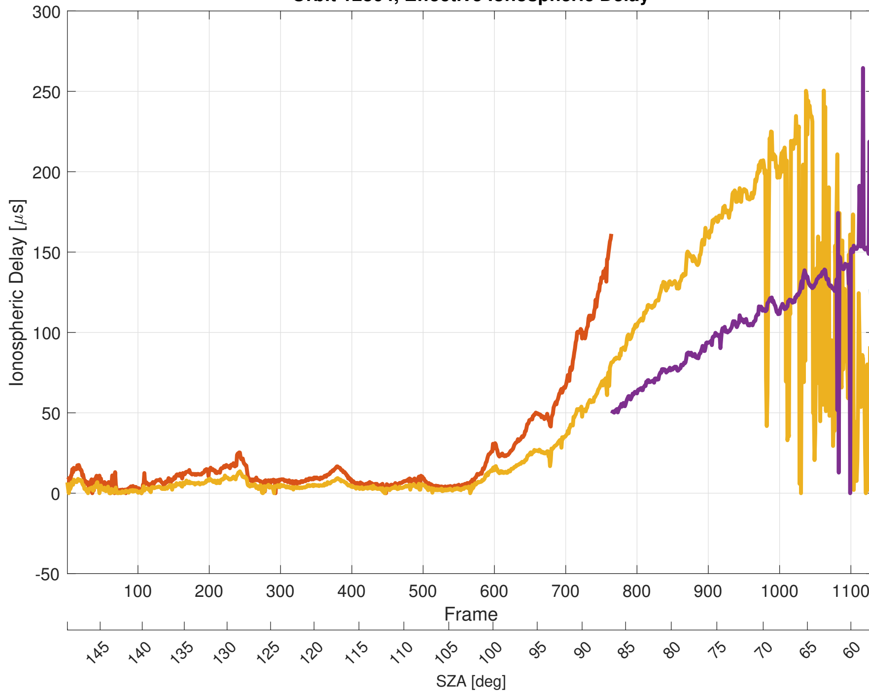
Orbit 12864, Effective Ionospheric Delay
