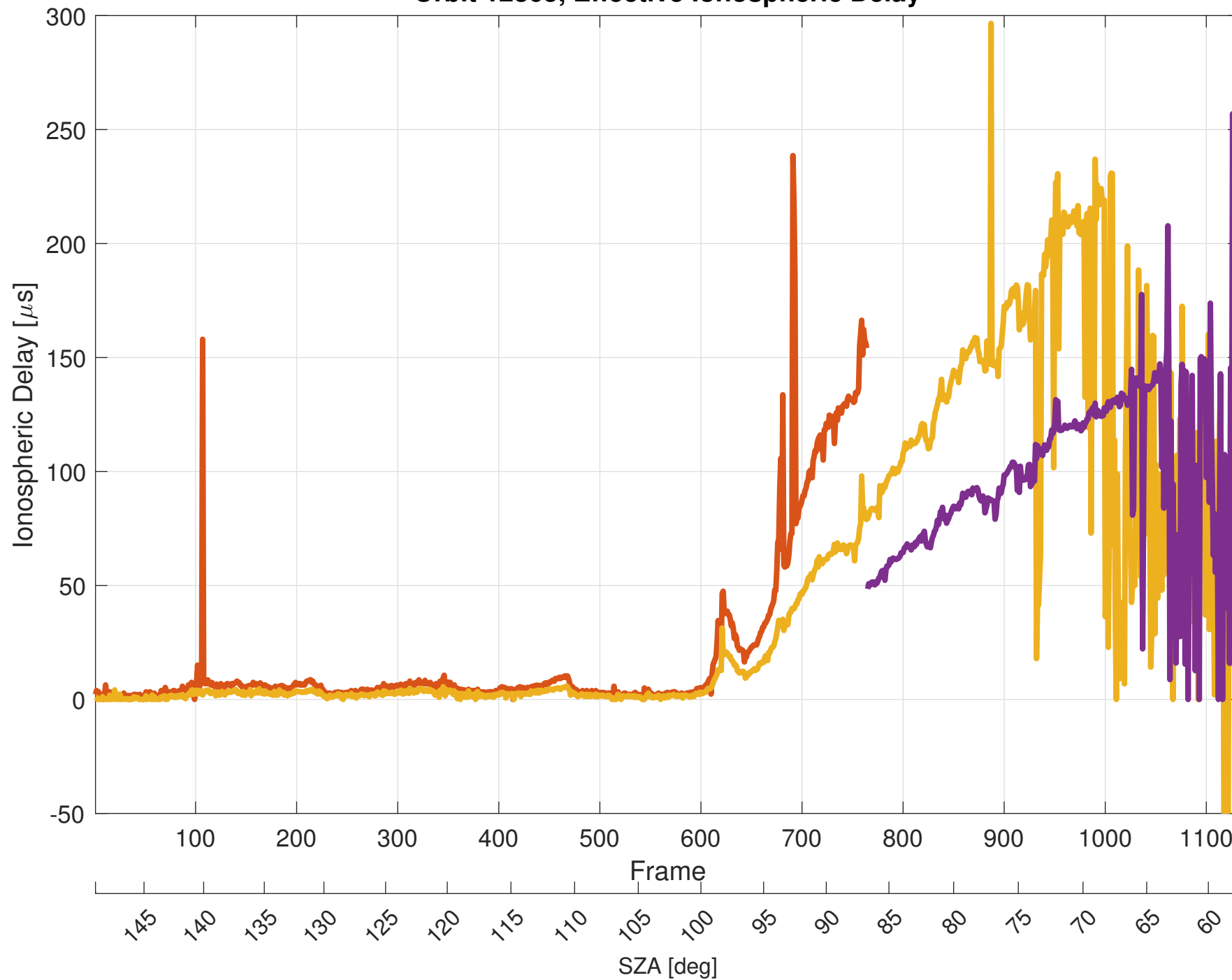
Orbit 12865, Effective Ionospheric Delay
