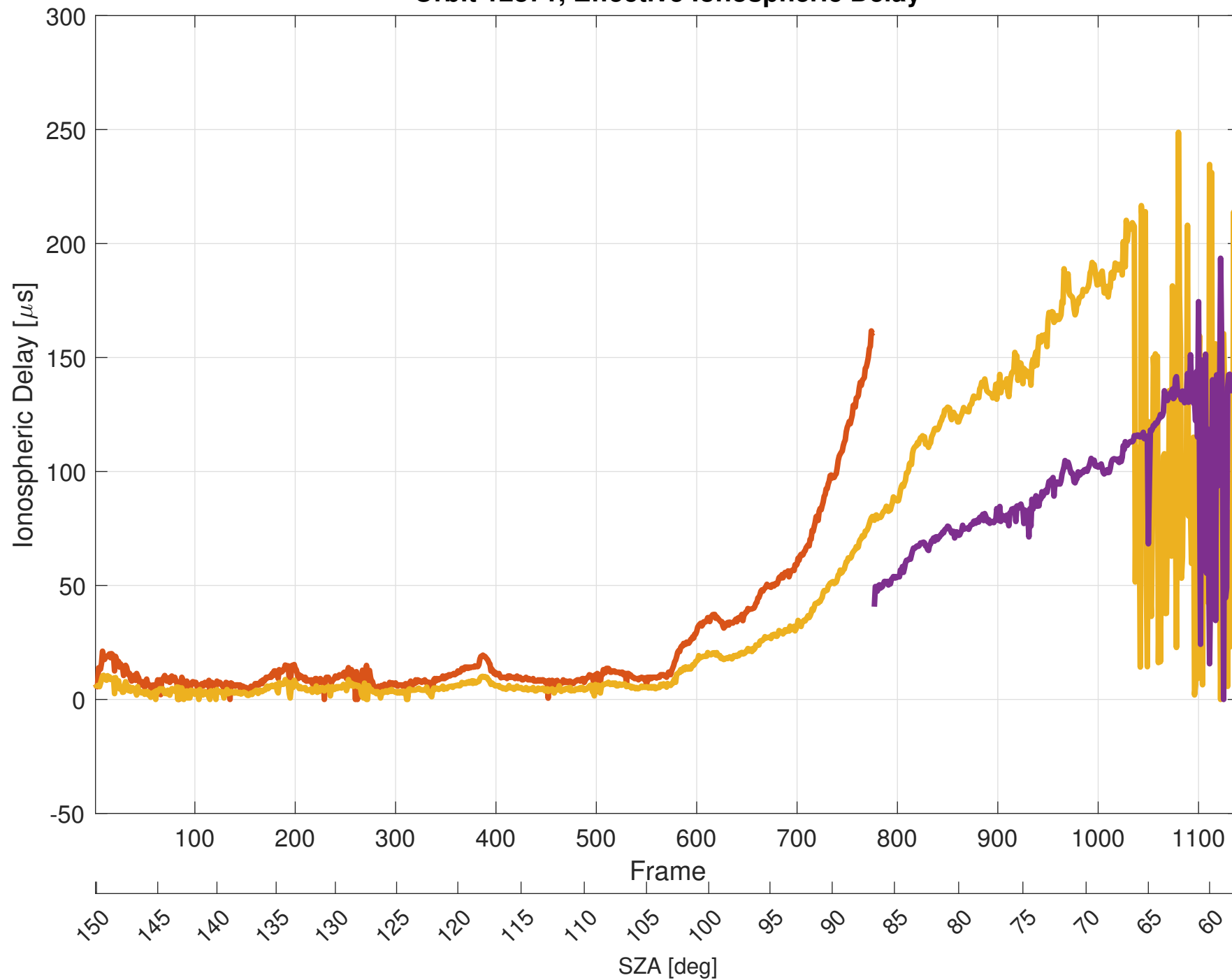
Orbit 12871, Effective Ionospheric Delay
