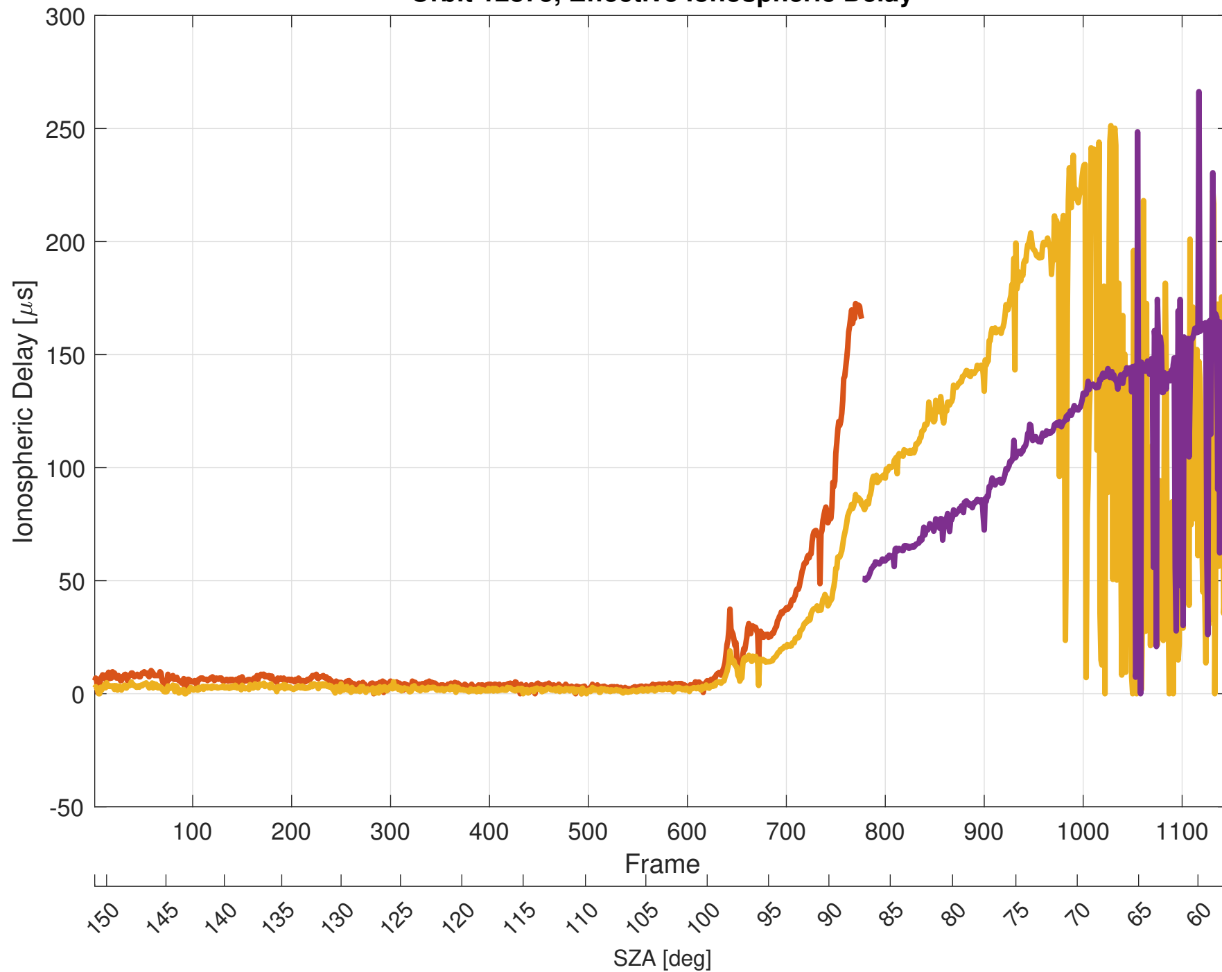
Orbit 12875, Effective Ionospheric Delay
