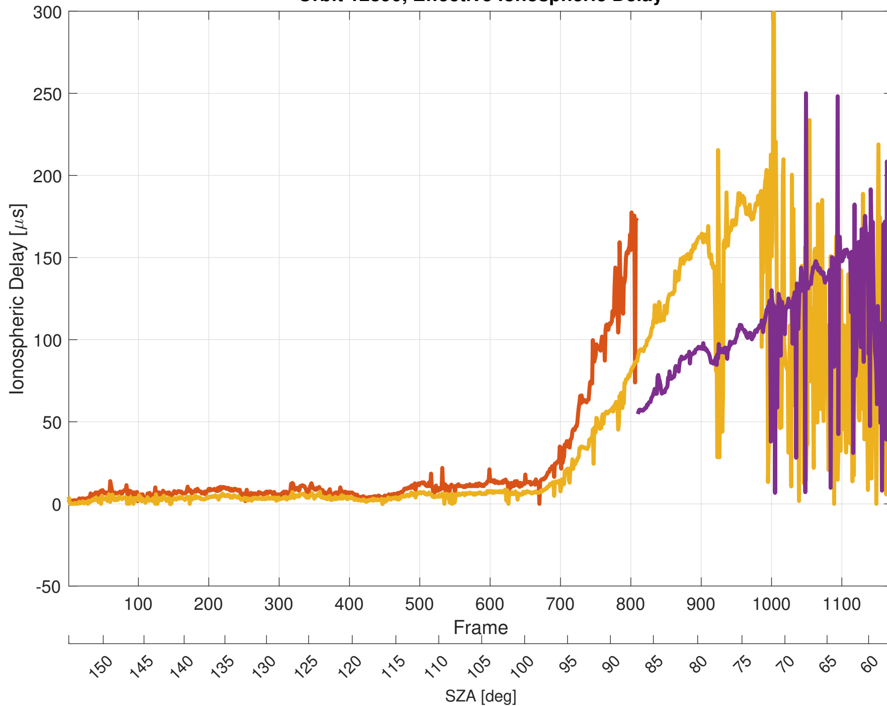
Orbit 12890, Effective Ionospheric Delay
