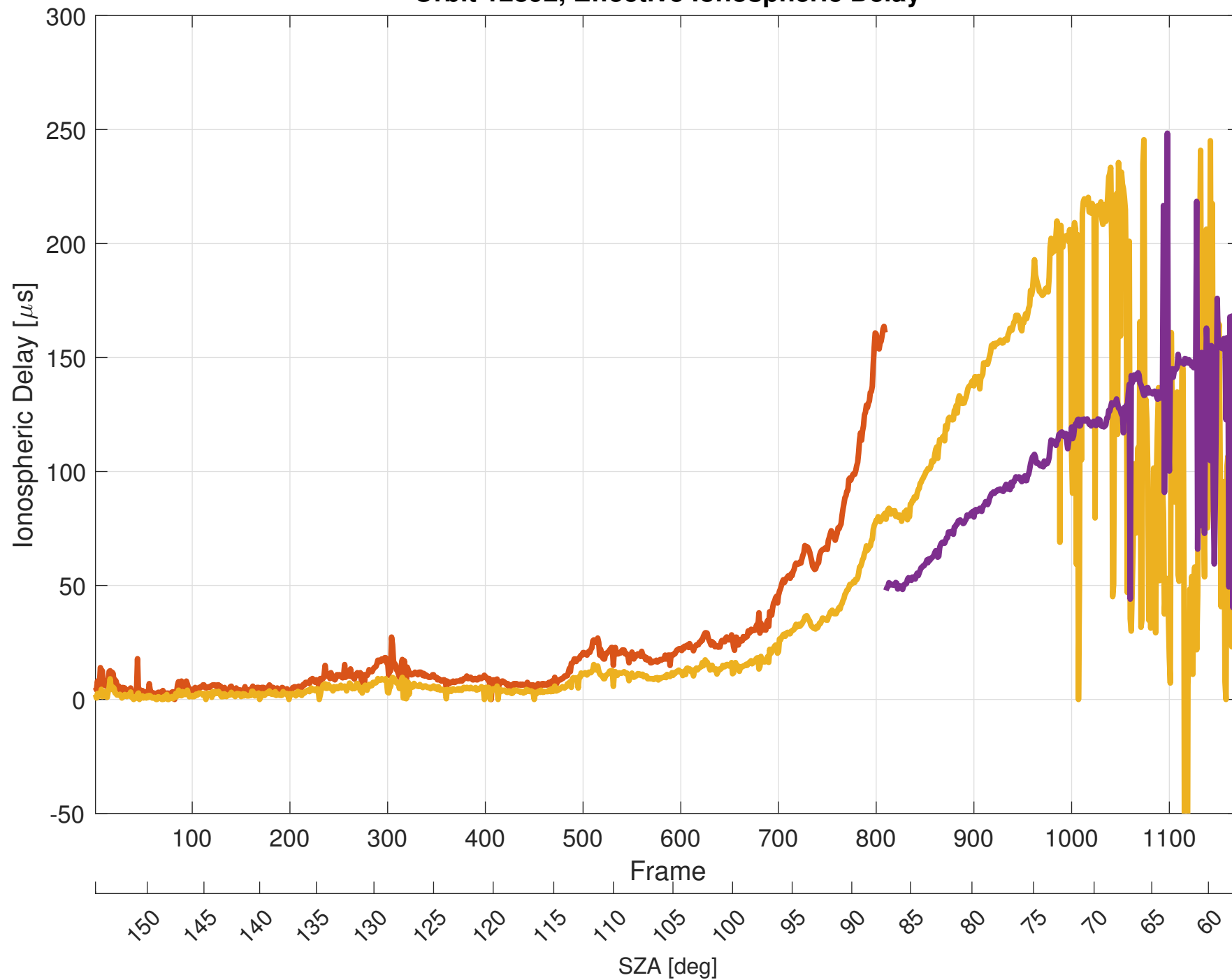
Orbit 12892, Effective Ionospheric Delay
