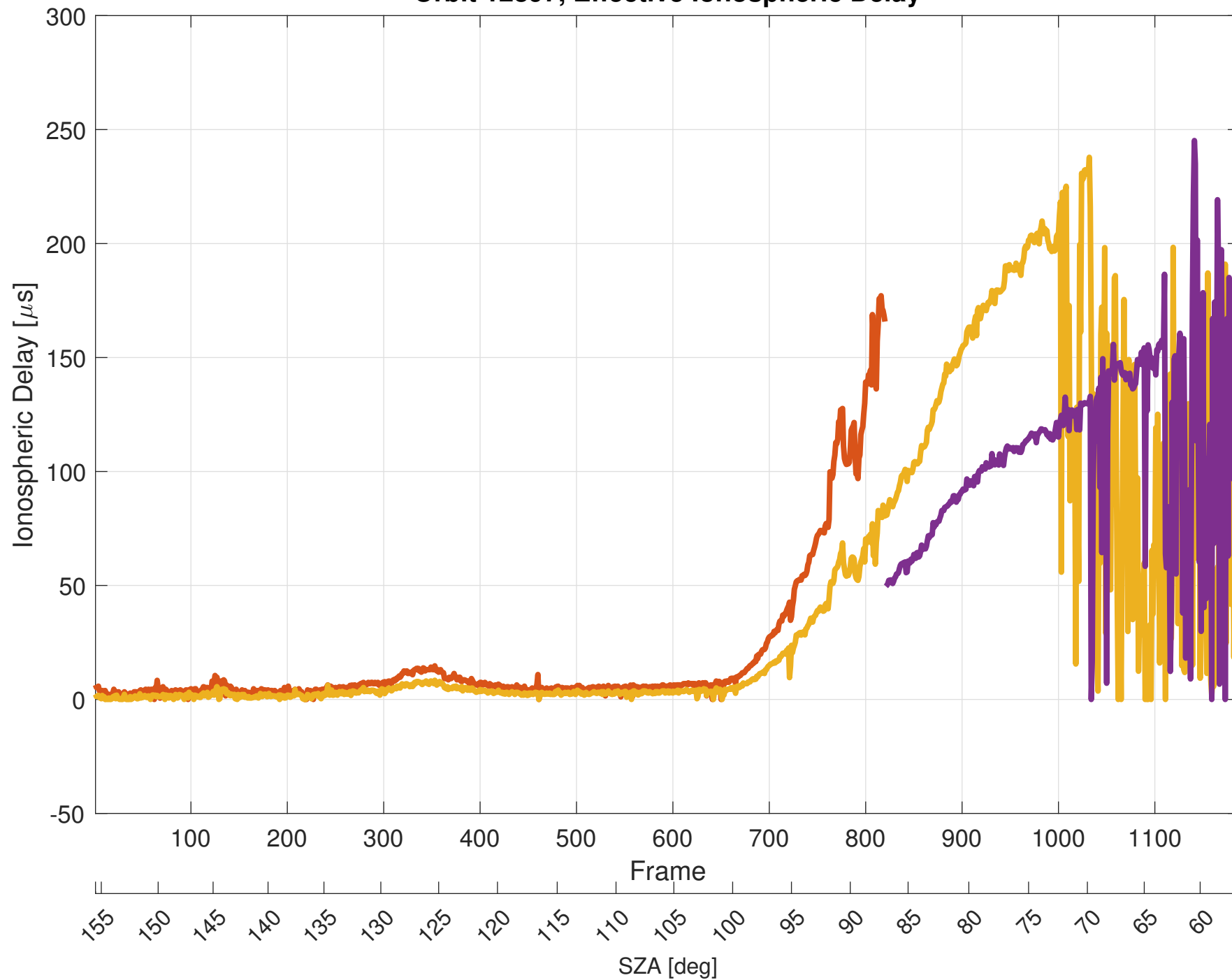
Orbit 12897, Effective Ionospheric Delay
