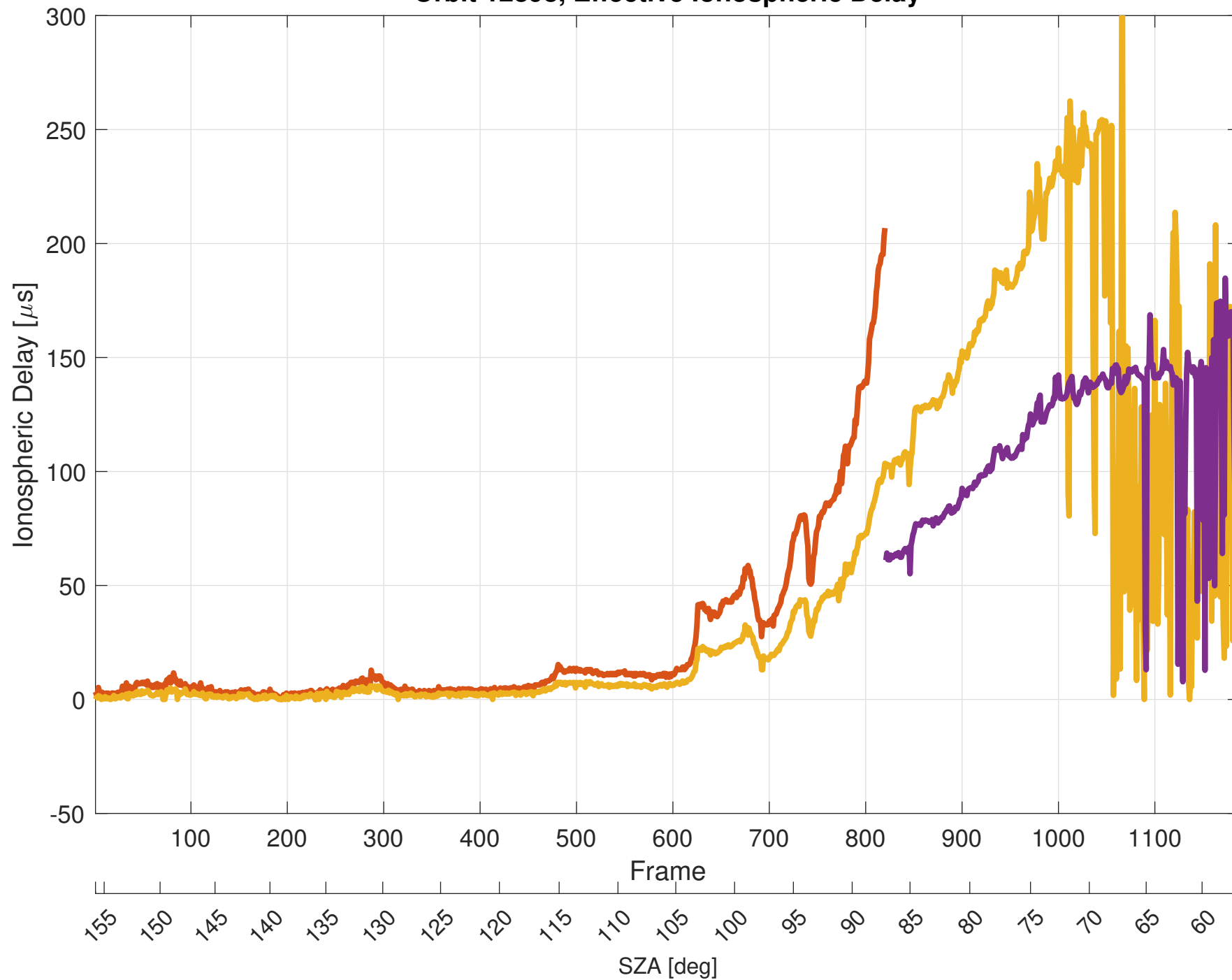
Orbit 12898, Effective Ionospheric Delay
