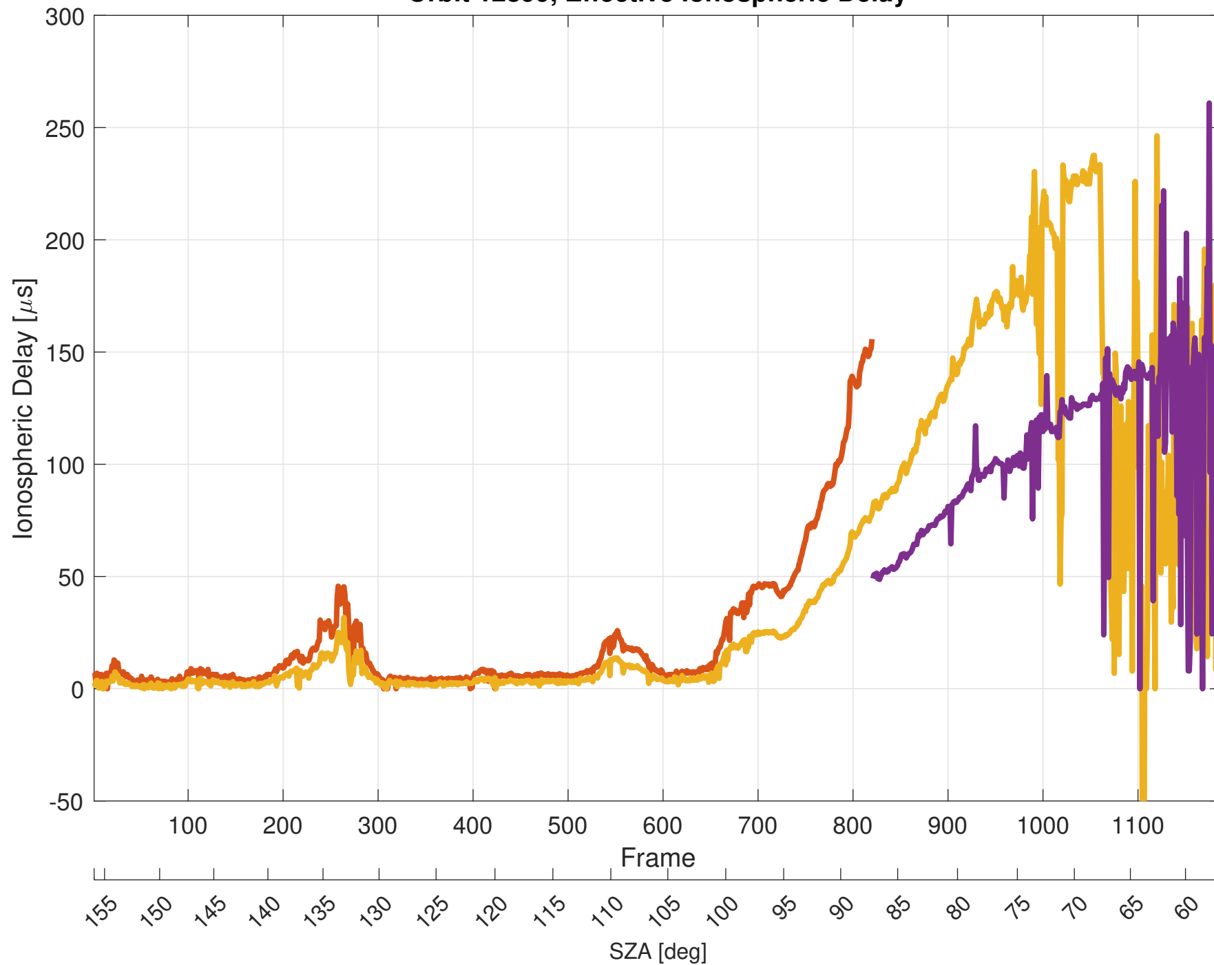
Orbit 12899, Effective Ionospheric Delay
