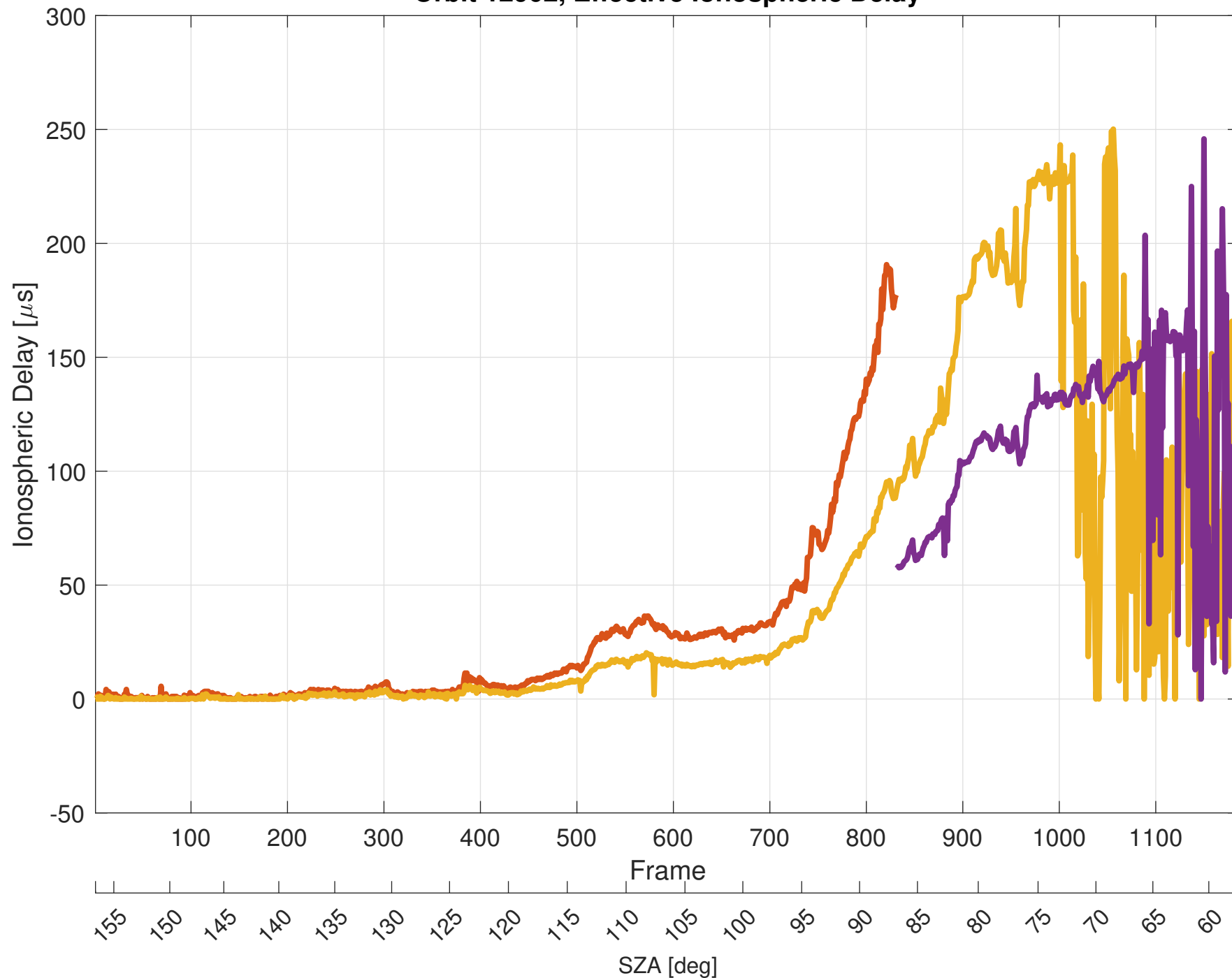
Orbit 12902, Effective Ionospheric Delay
