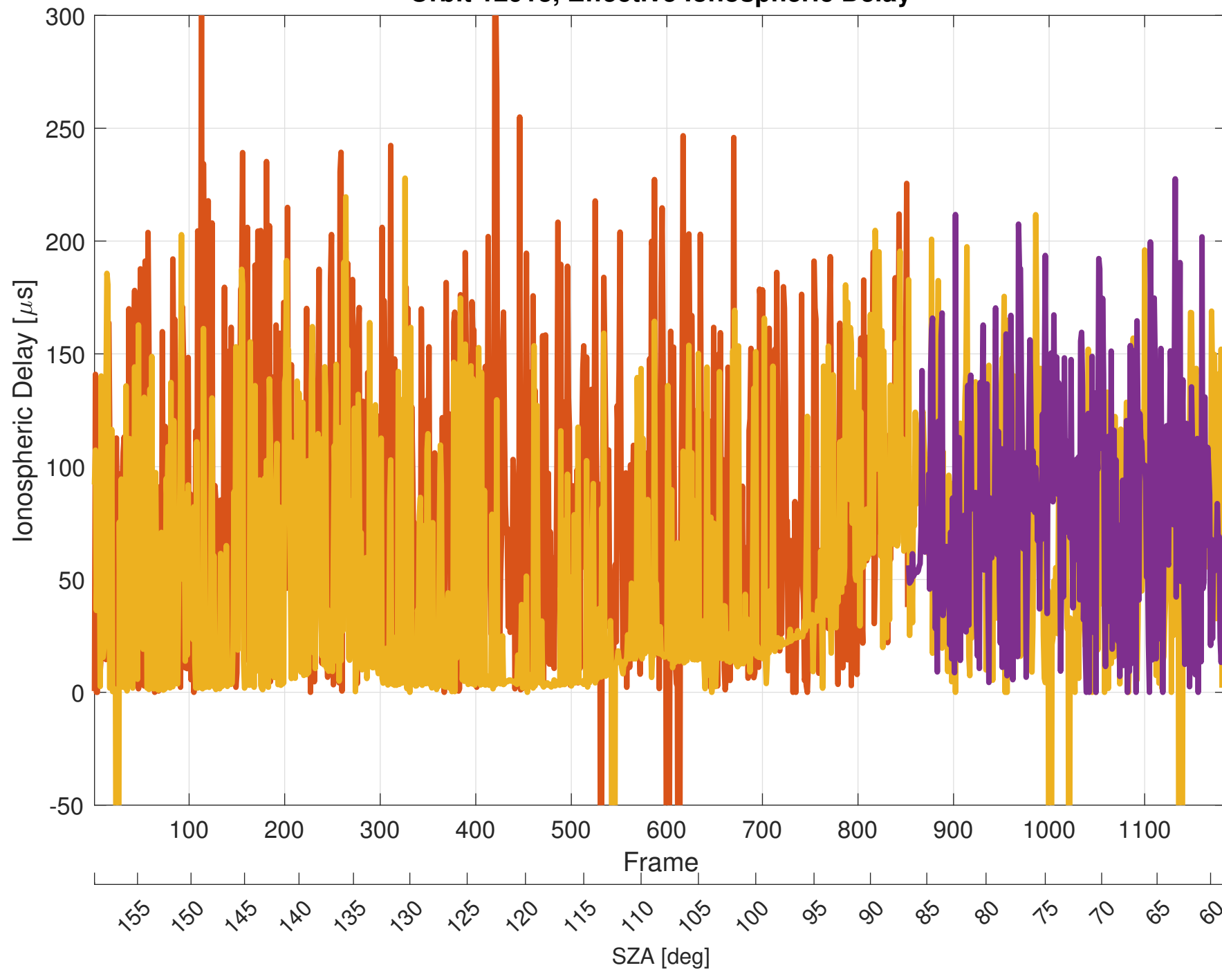
Orbit 12913, Effective Ionospheric Delay
