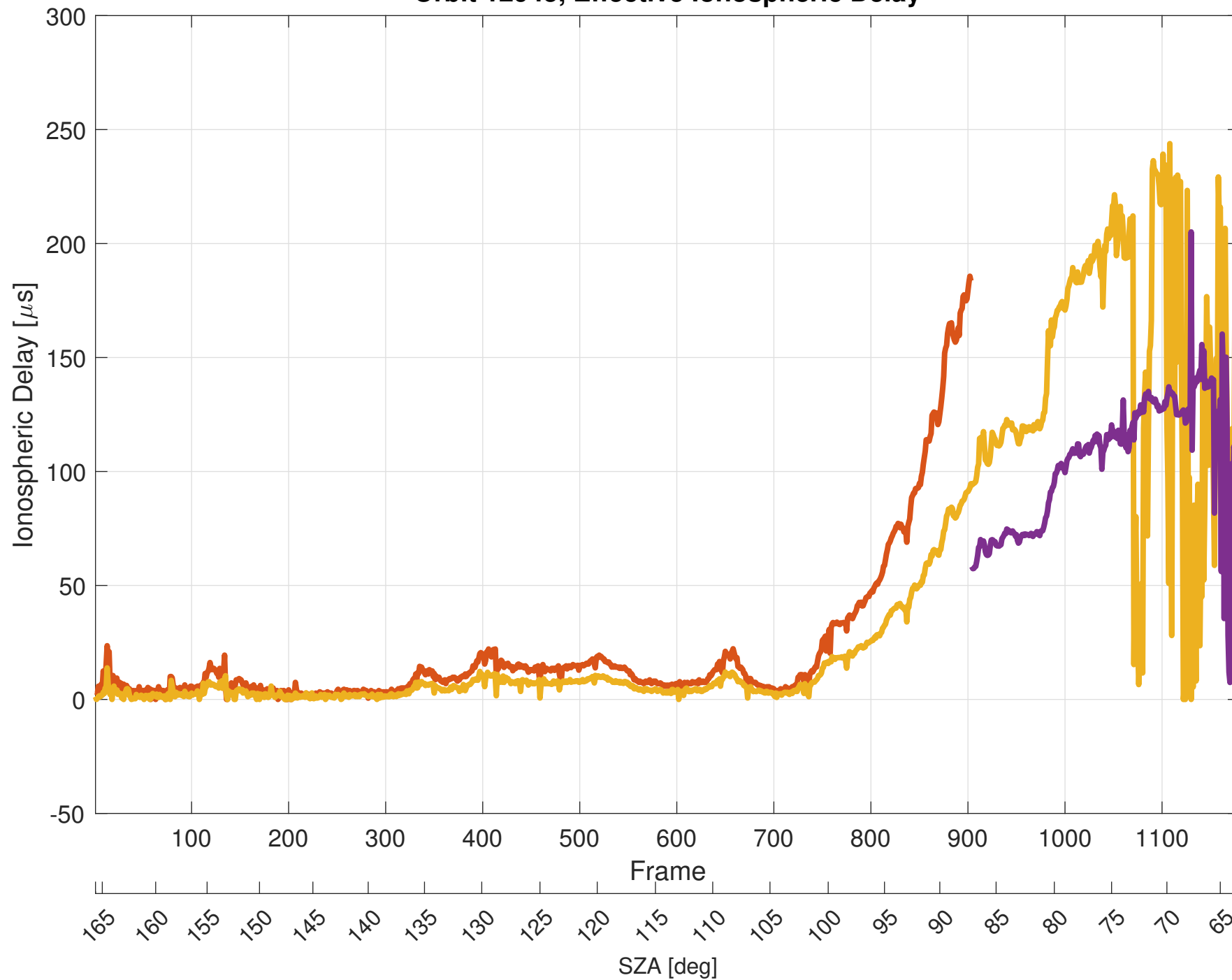
Orbit 12945, Effective Ionospheric Delay
