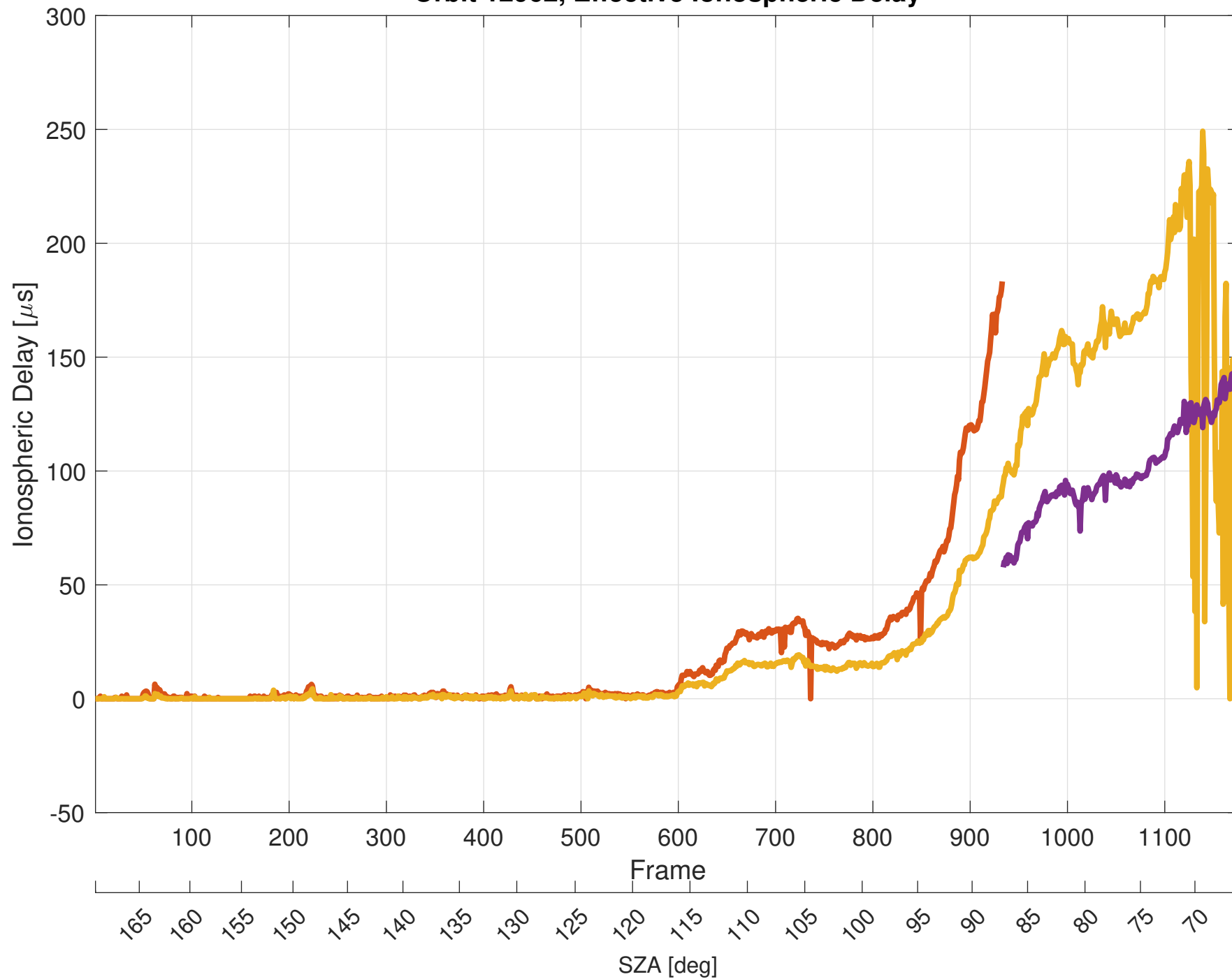
Orbit 12962, Effective Ionospheric Delay
