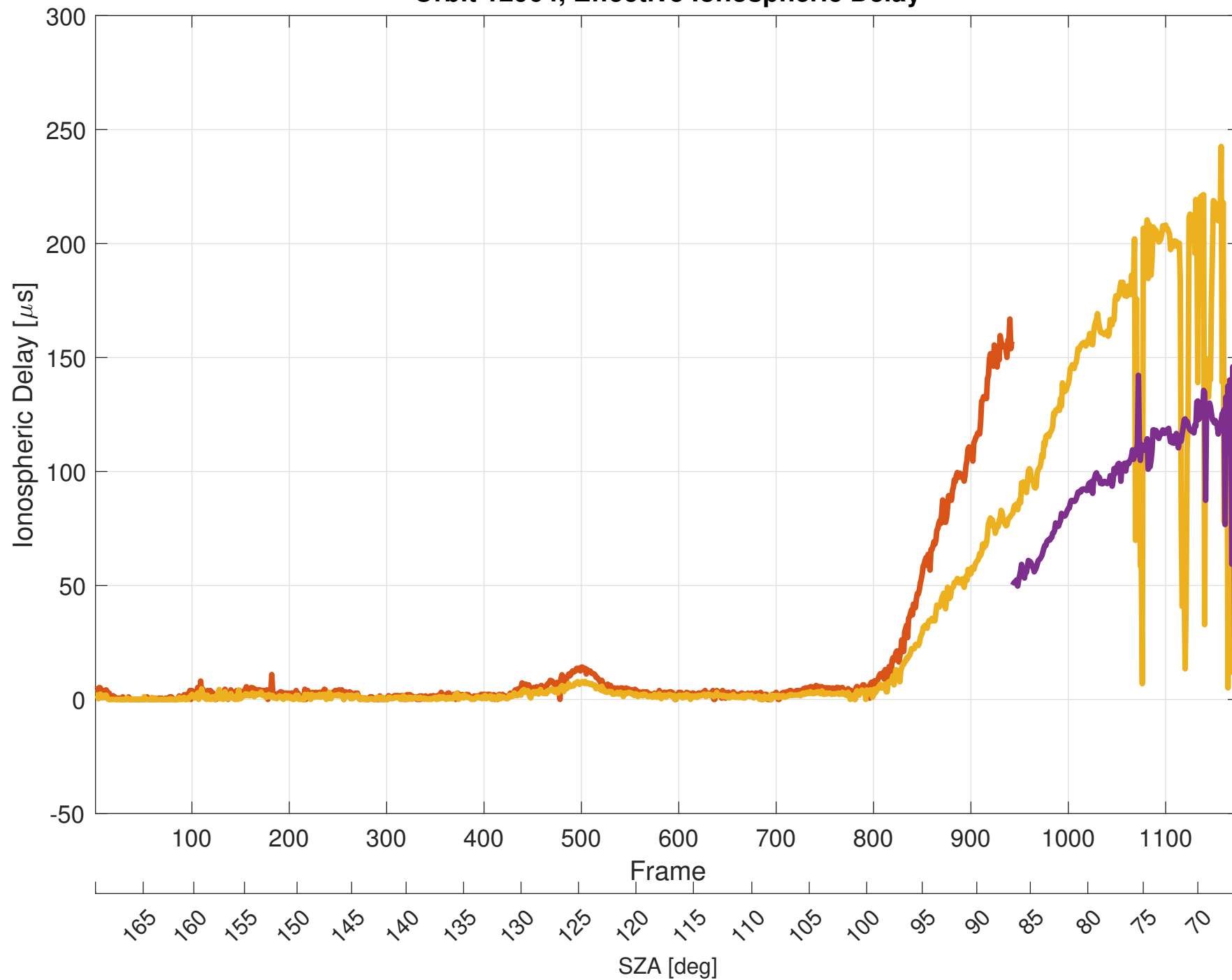
Orbit 12964, Effective Ionospheric Delay
