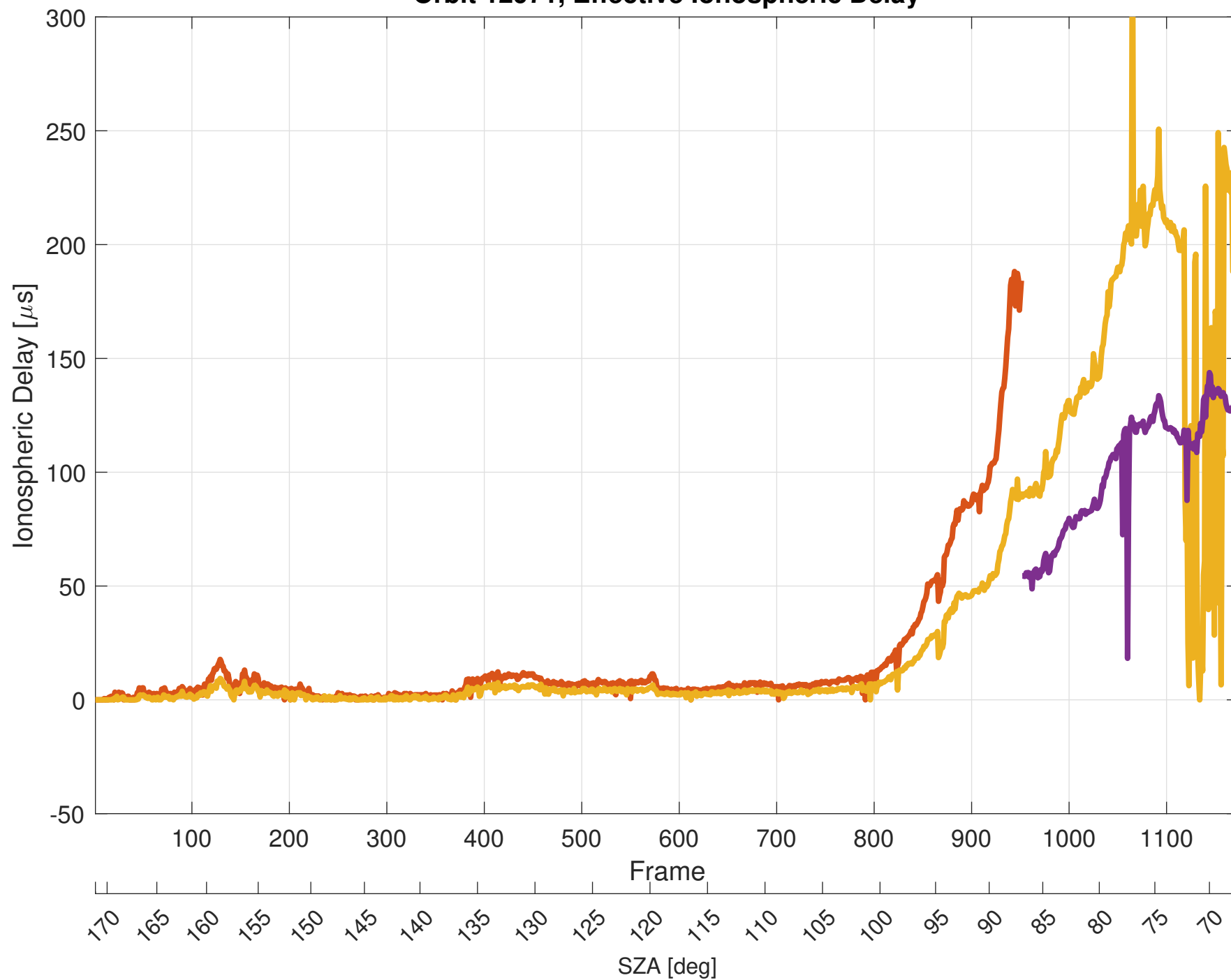
Orbit 12971, Effective Ionospheric Delay
