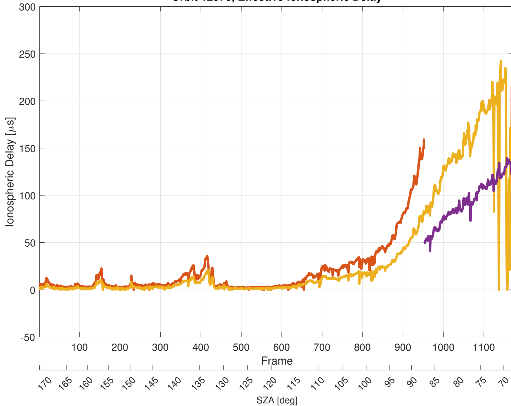
Orbit 12973, Effective Ionospheric Delay
