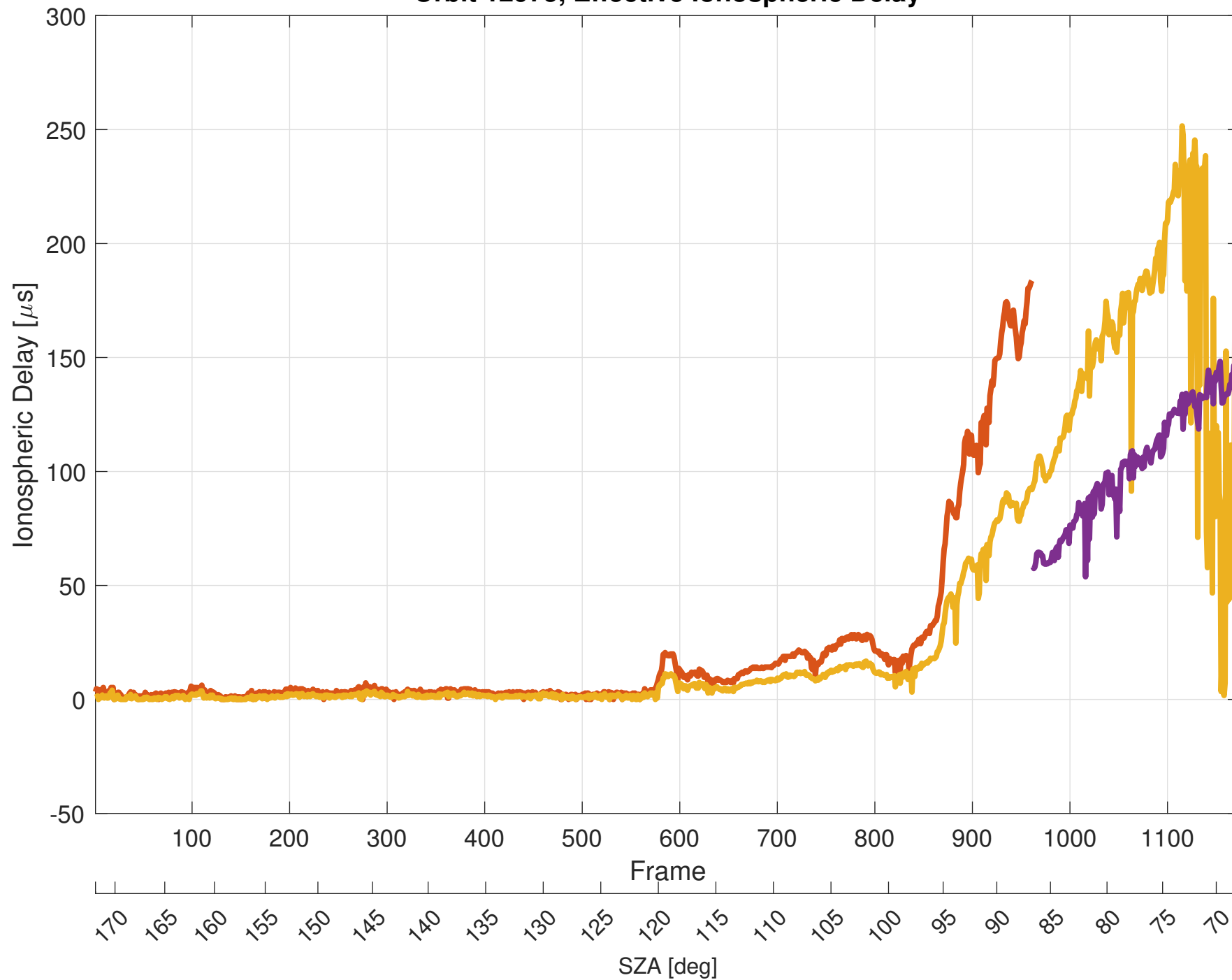
Orbit 12975, Effective Ionospheric Delay
