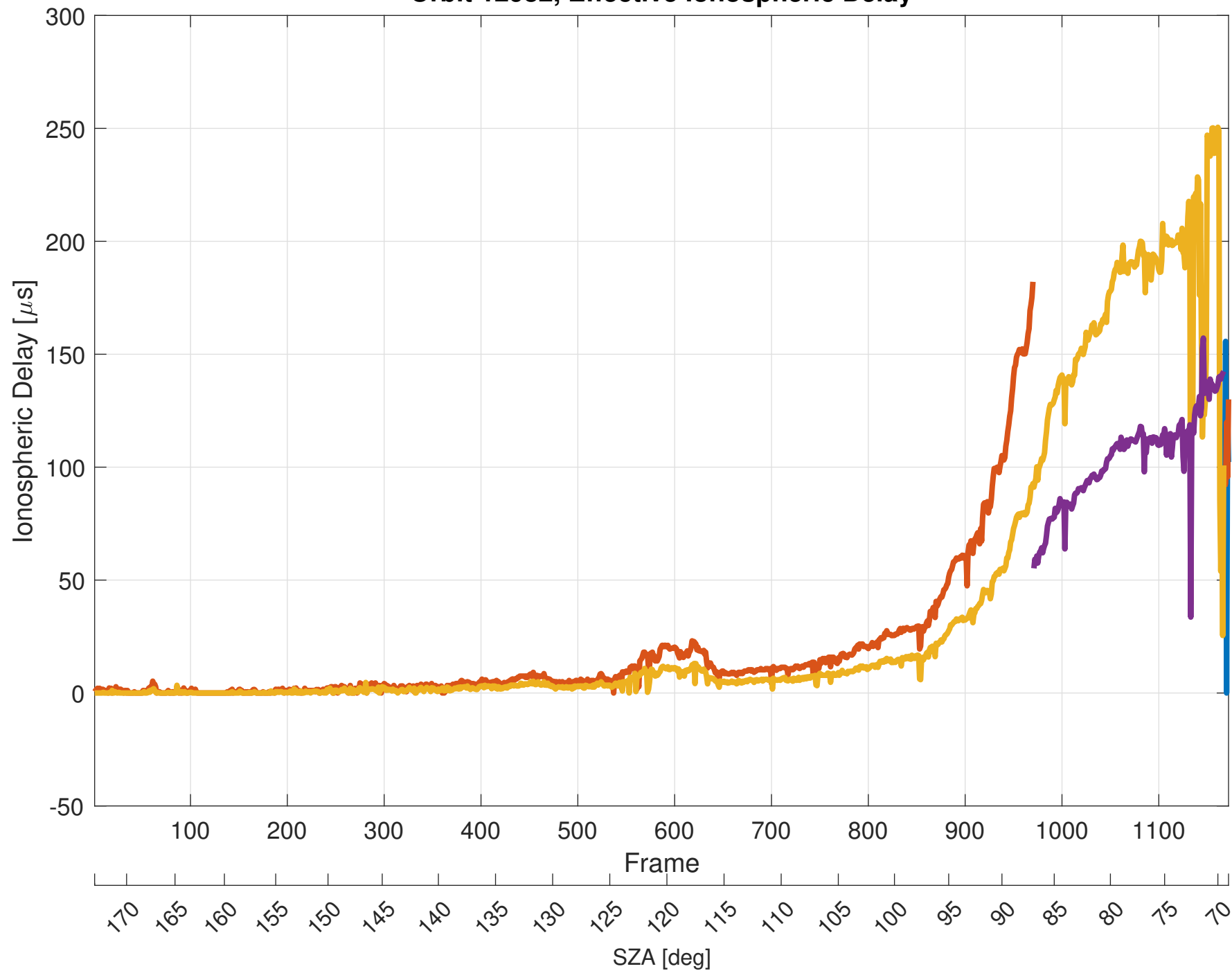
Orbit 12982, Effective Ionospheric Delay
