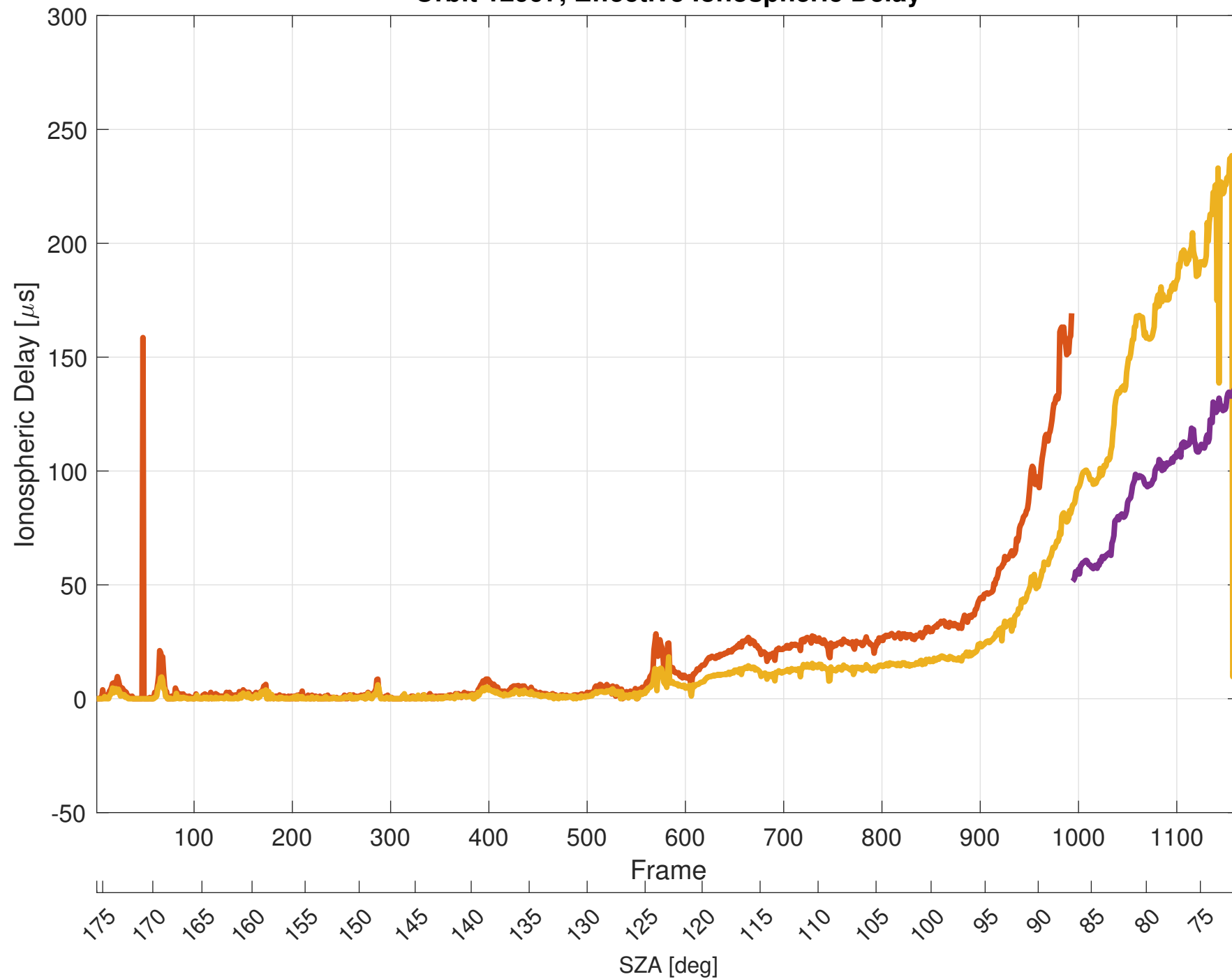
Orbit 12997, Effective Ionospheric Delay
