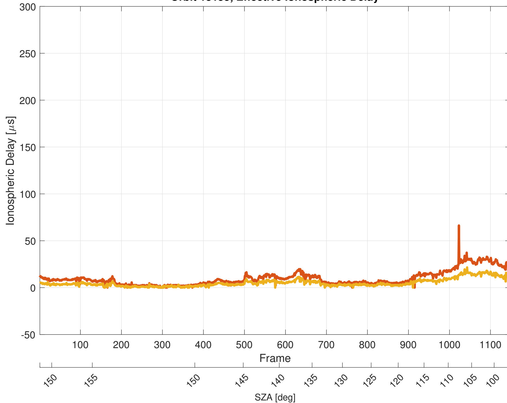
Orbit 13155, Effective Ionospheric Delay
