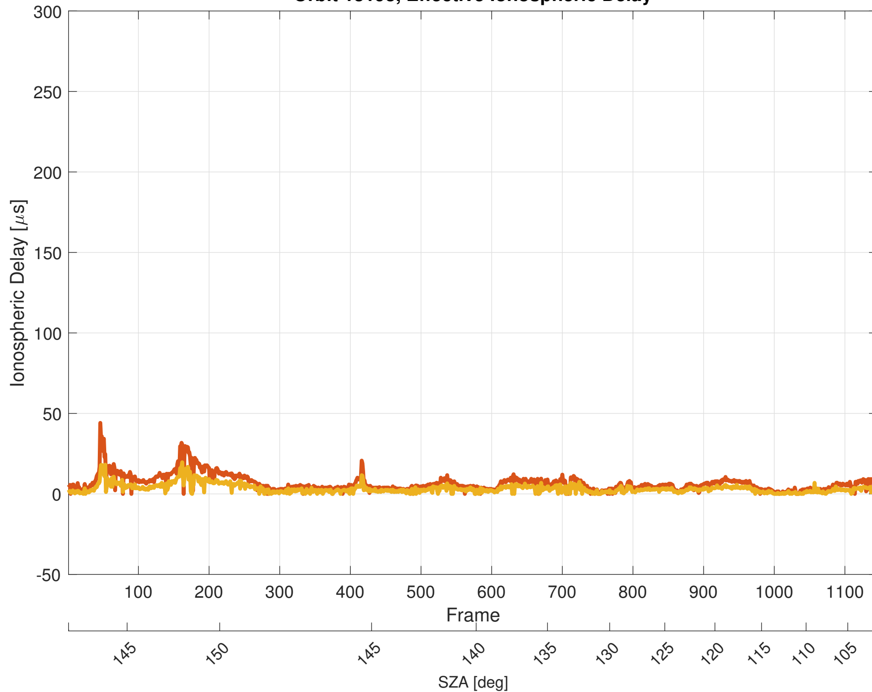
Orbit 13193, Effective Ionospheric Delay
