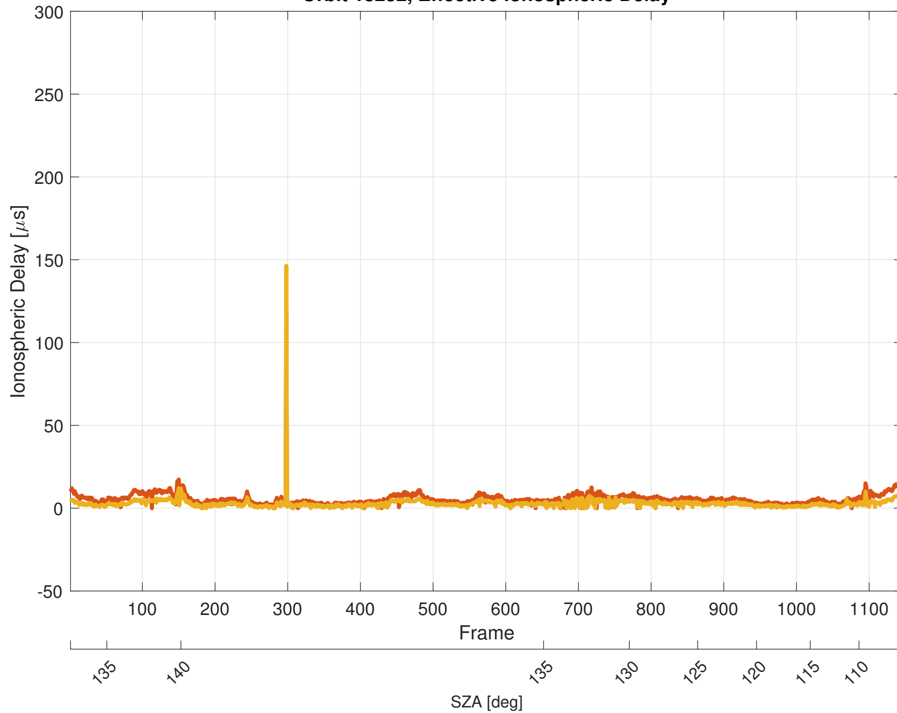
Orbit 13232, Effective Ionospheric Delay
