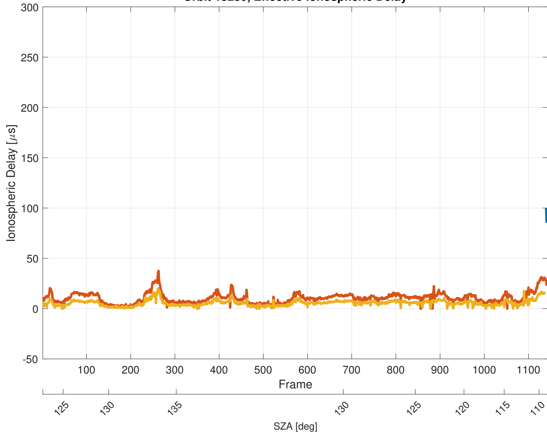
Orbit 13280, Effective Ionospheric Delay
