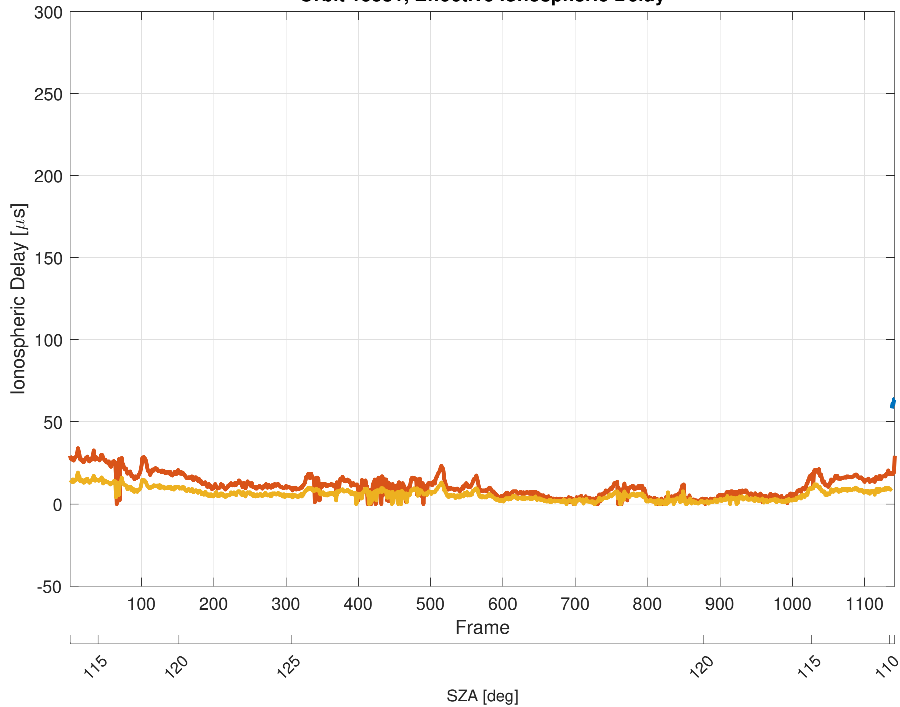
Orbit 13331, Effective Ionospheric Delay
