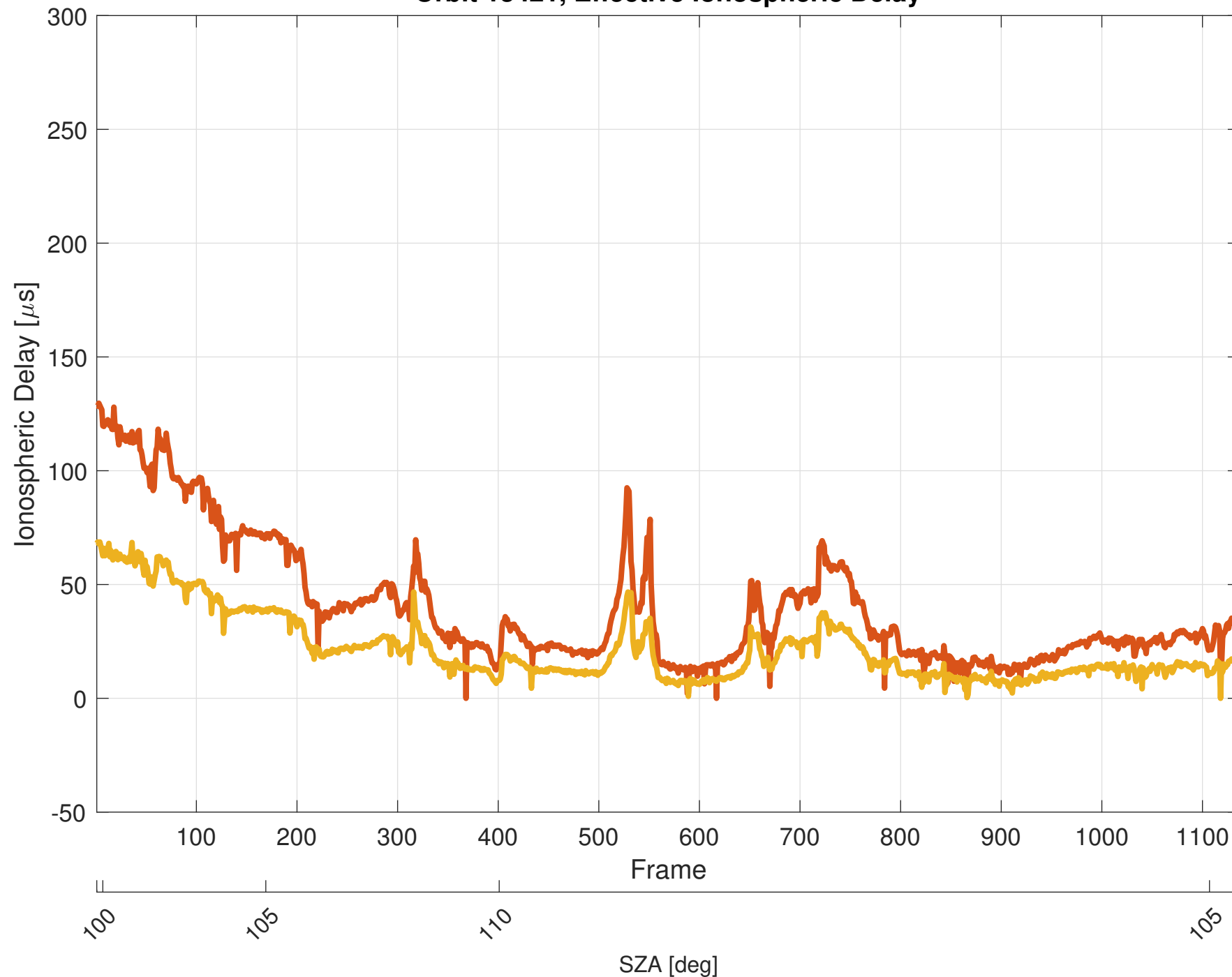
Orbit 13421, Effective Ionospheric Delay
