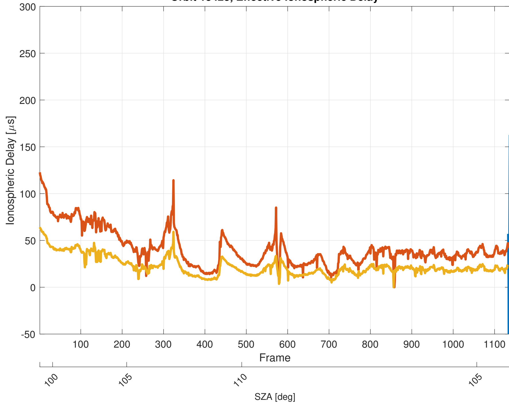
Orbit 13428, Effective Ionospheric Delay
