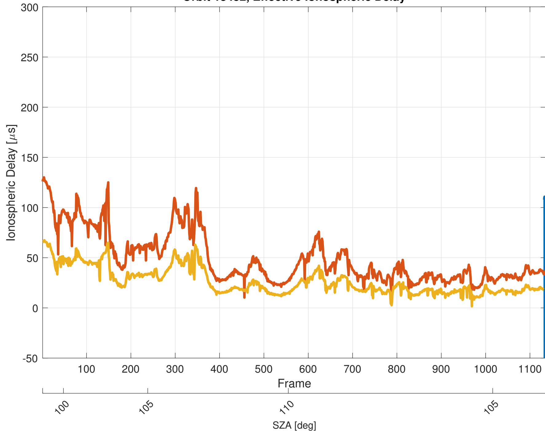
Orbit 13432, Effective Ionospheric Delay
