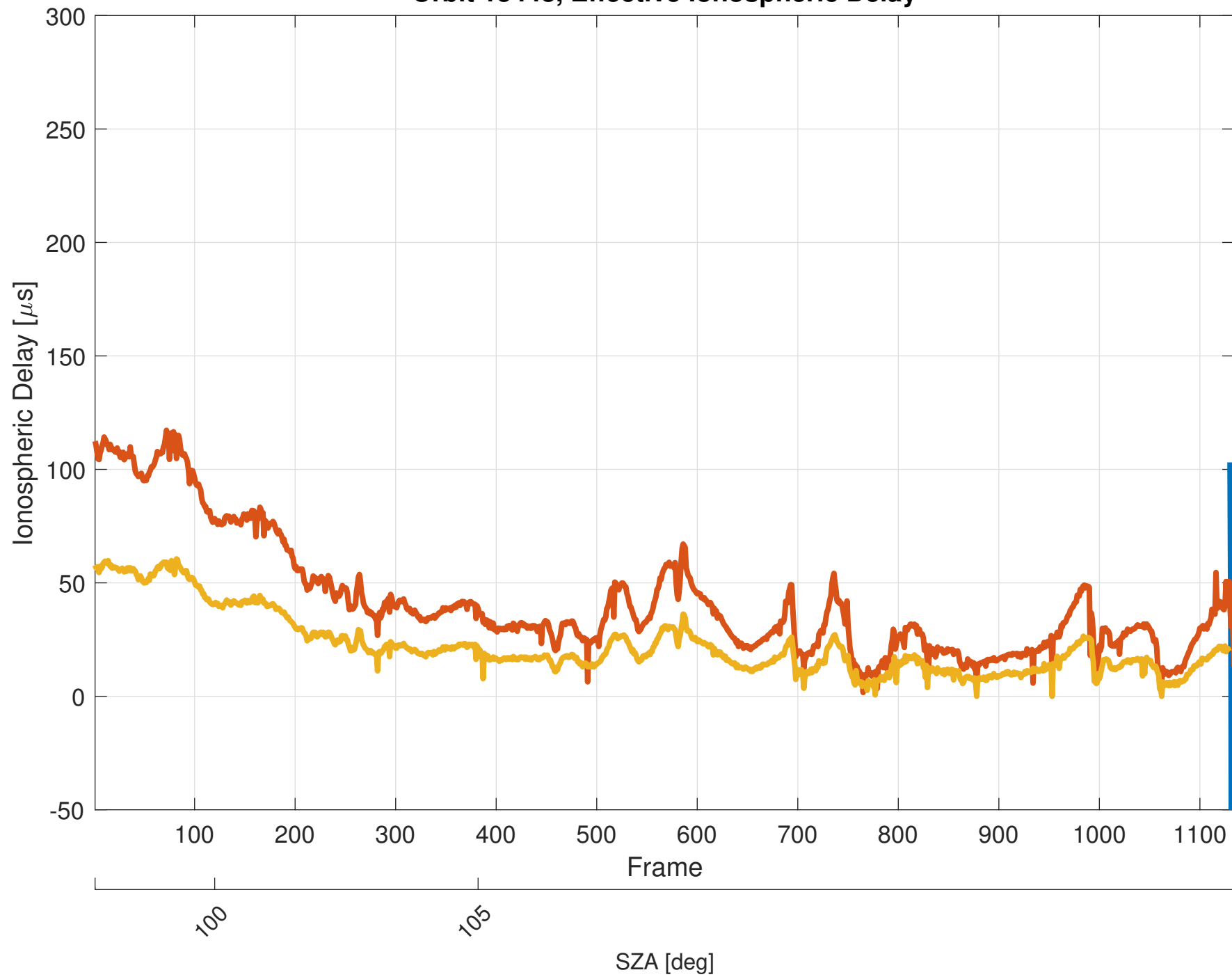
Orbit 13448, Effective Ionospheric Delay
