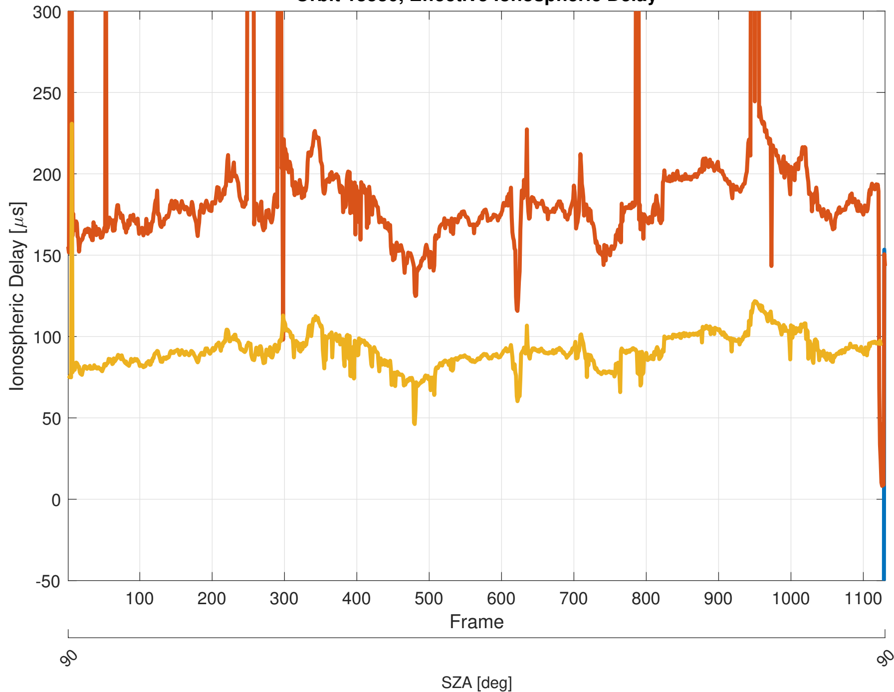
Orbit 13530, Effective Ionospheric Delay
