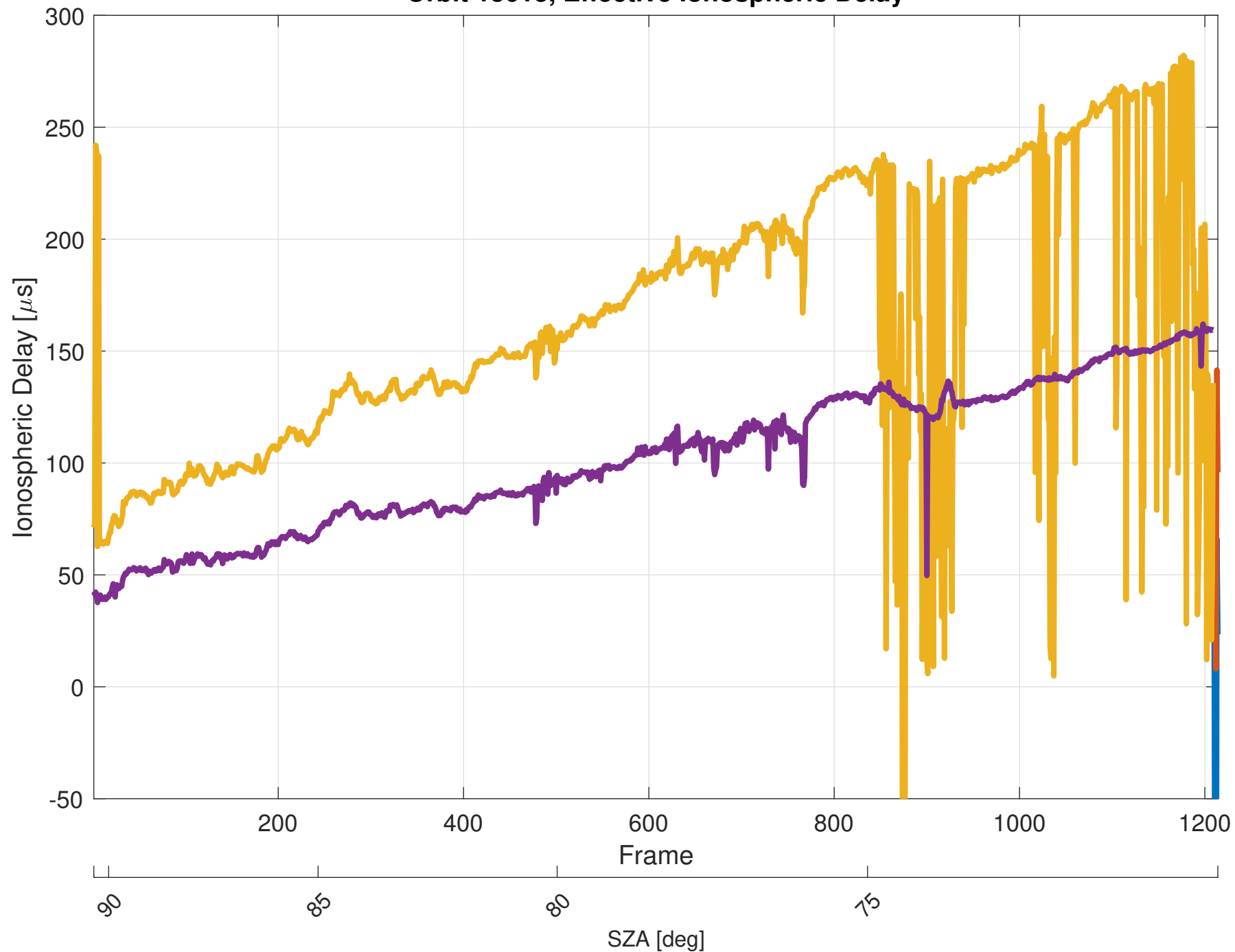
Orbit 13613, Effective Ionospheric Delay
