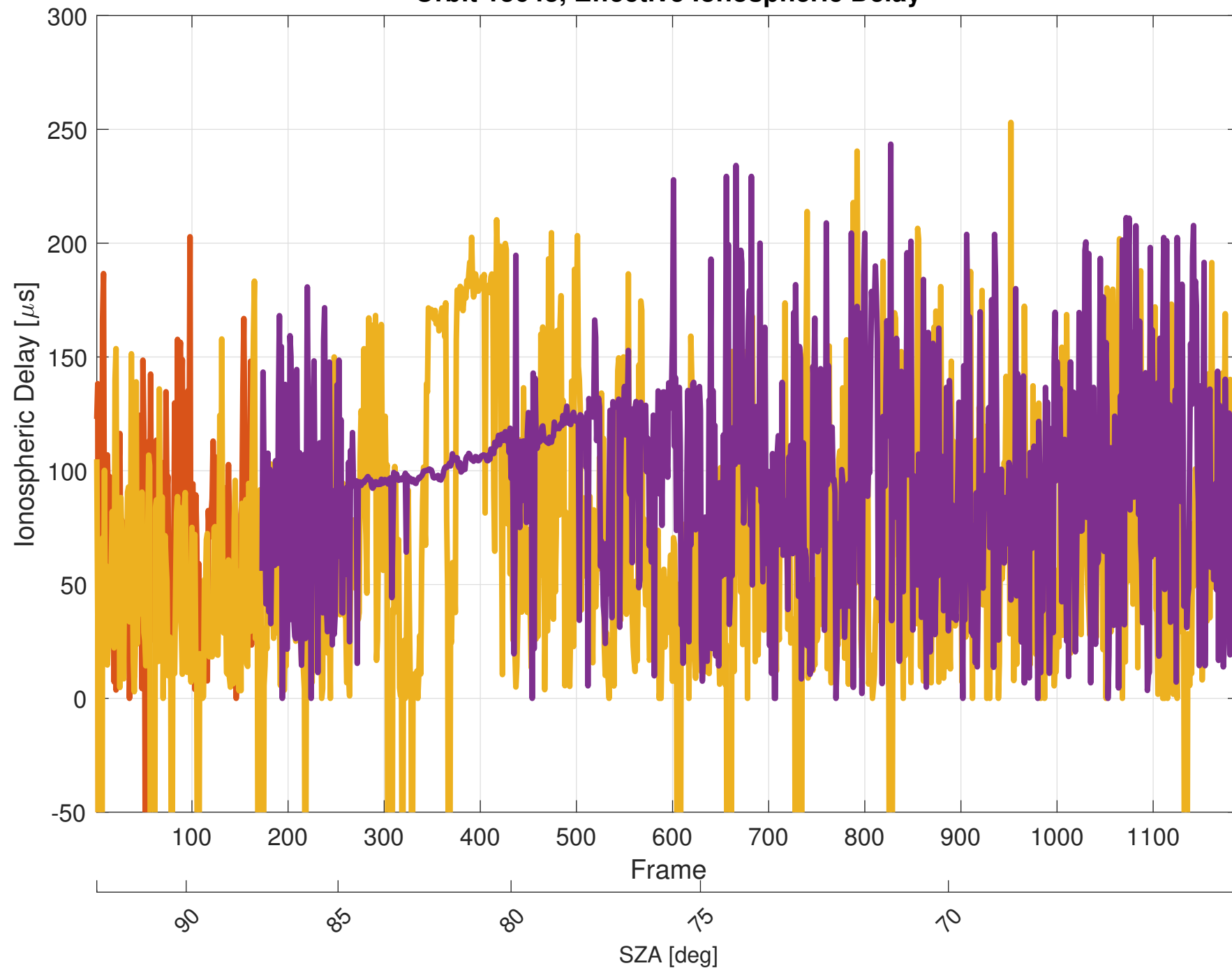
Orbit 13643, Effective Ionospheric Delay
