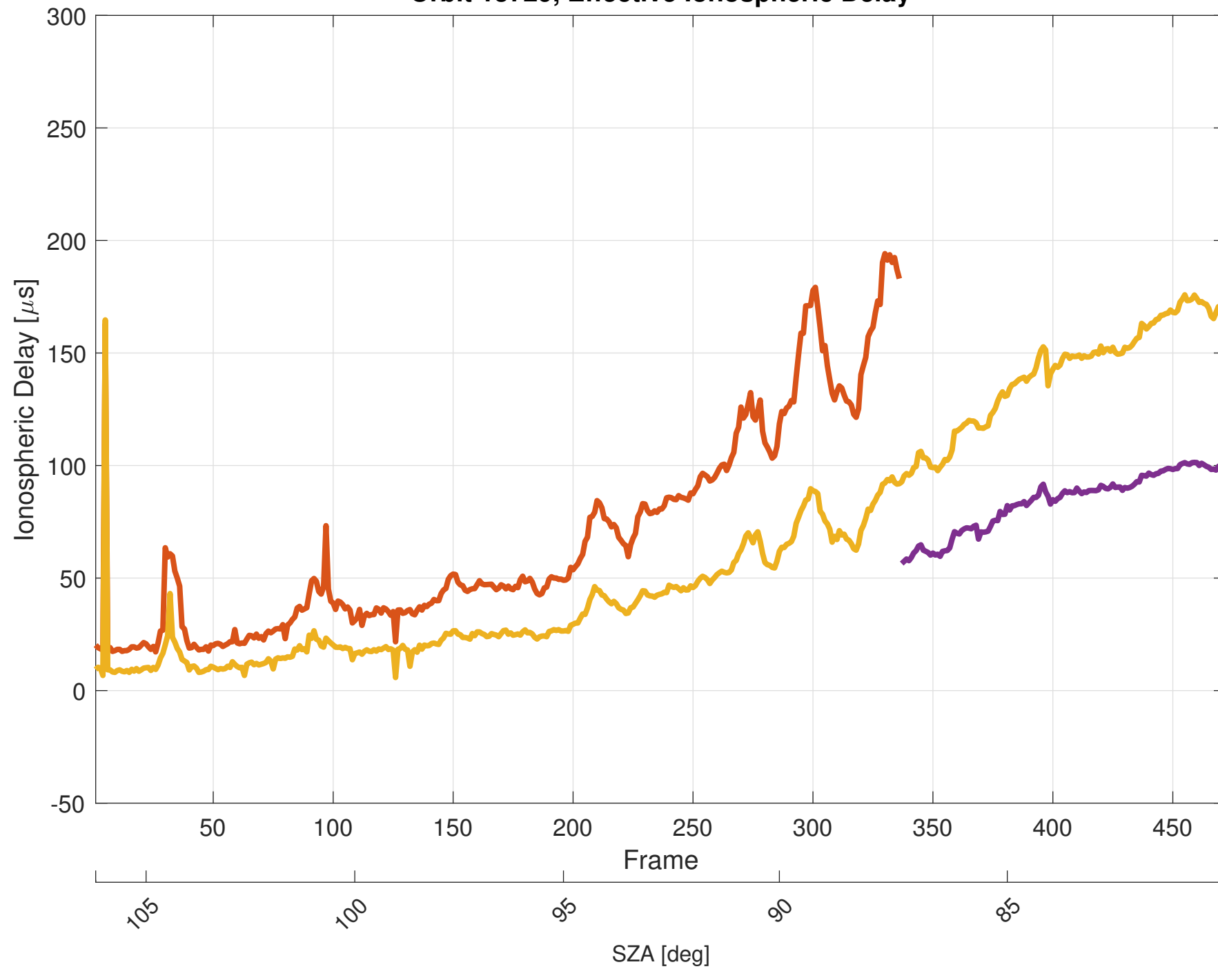
Orbit 13729, Effective Ionospheric Delay
