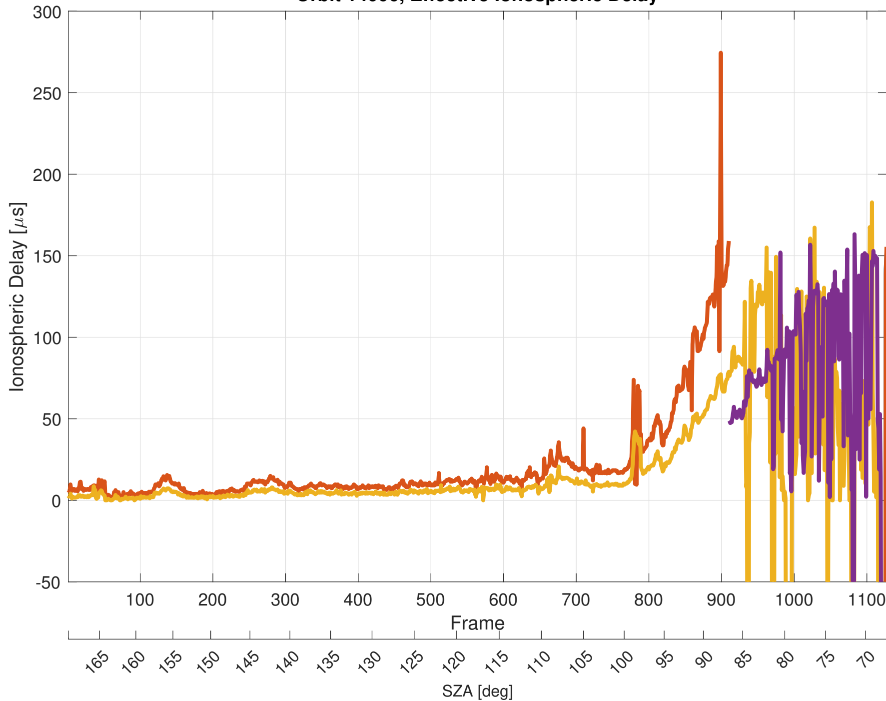
Orbit 14006, Effective Ionospheric Delay
