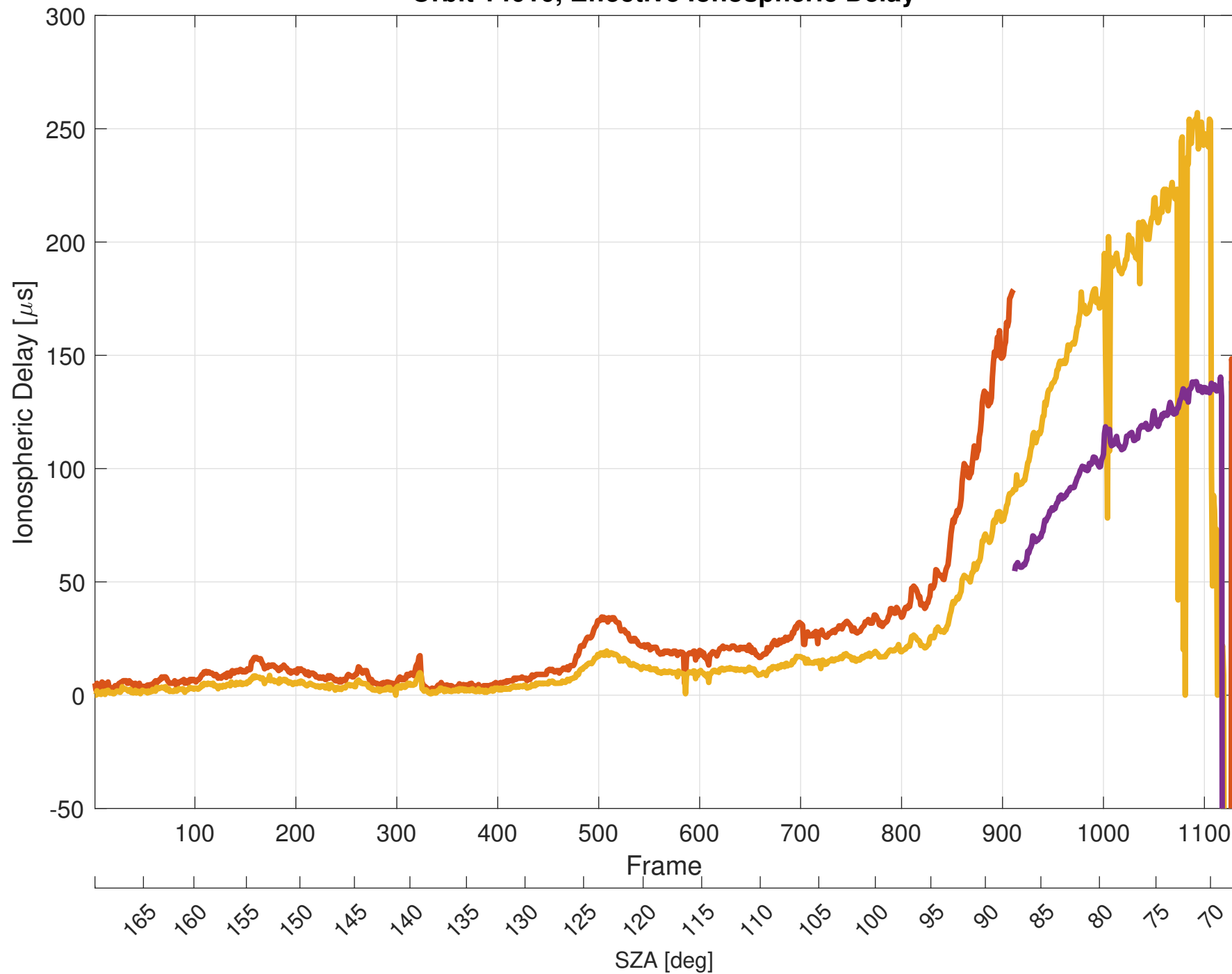
Orbit 14010, Effective Ionospheric Delay
