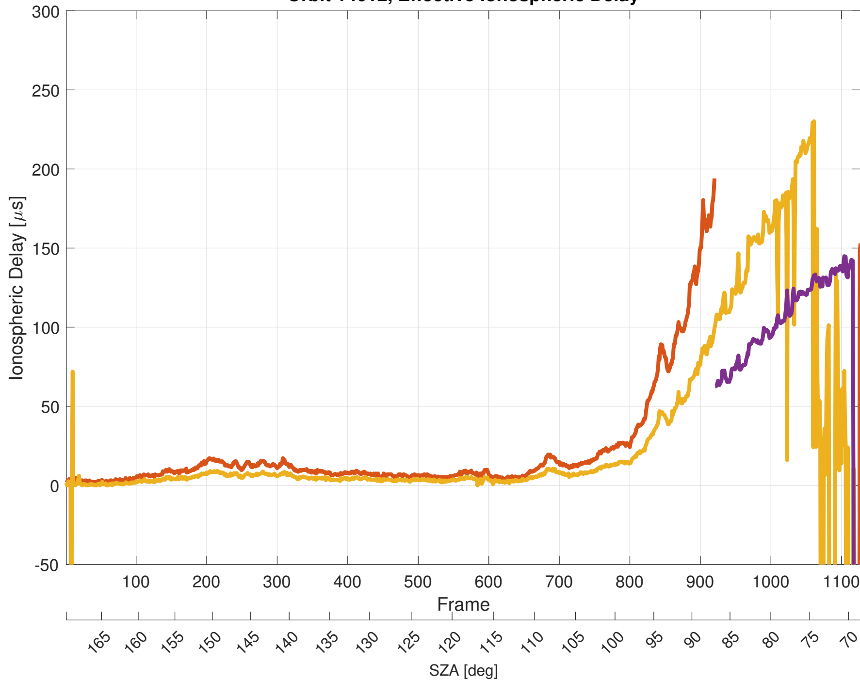
Orbit 14012, Effective Ionospheric Delay
