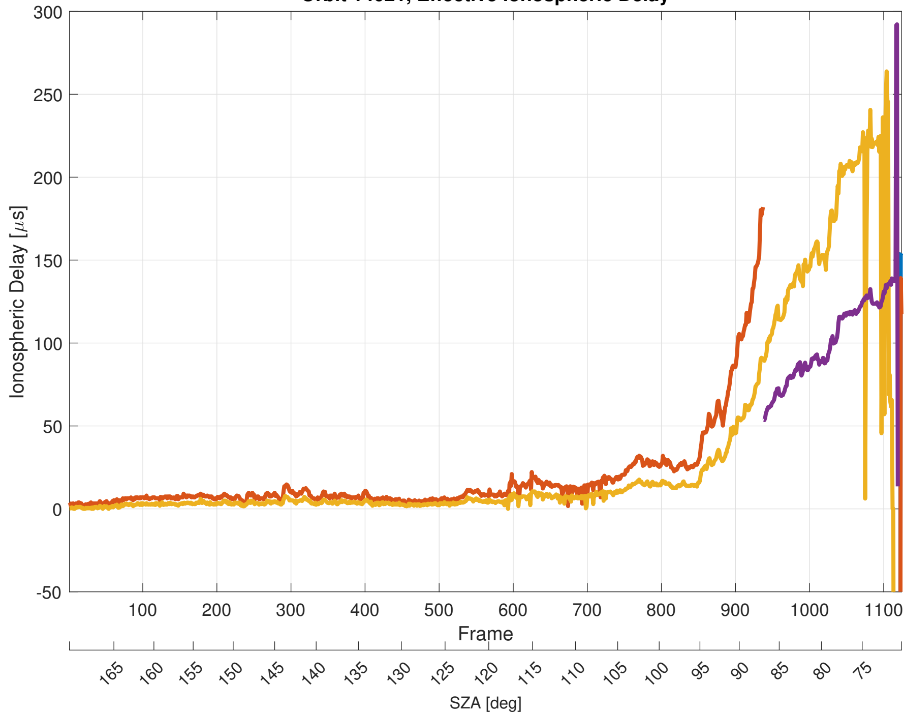
Orbit 14021, Effective Ionospheric Delay
