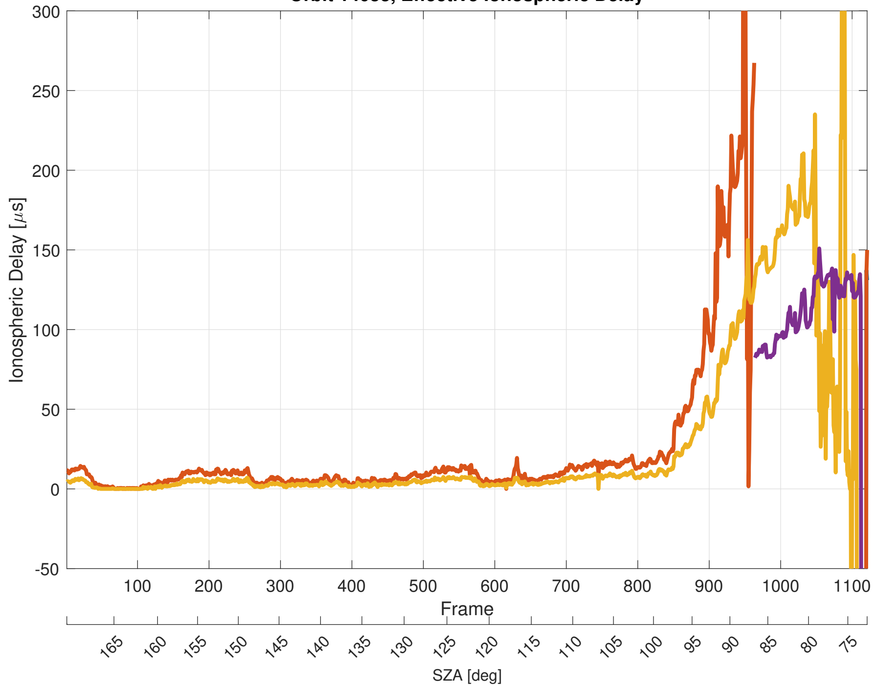
Orbit 14033, Effective Ionospheric Delay
