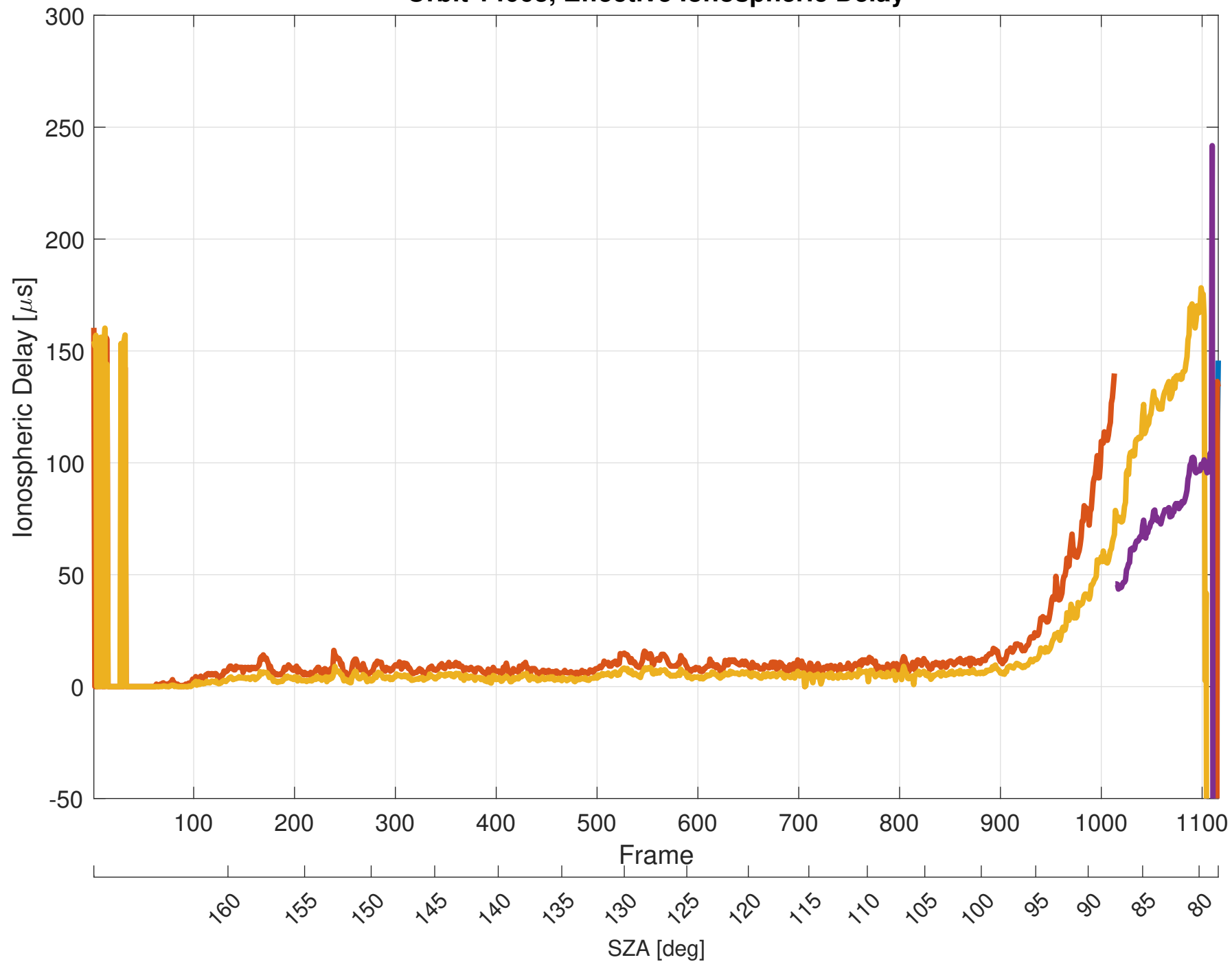
Orbit 14063, Effective Ionospheric Delay
