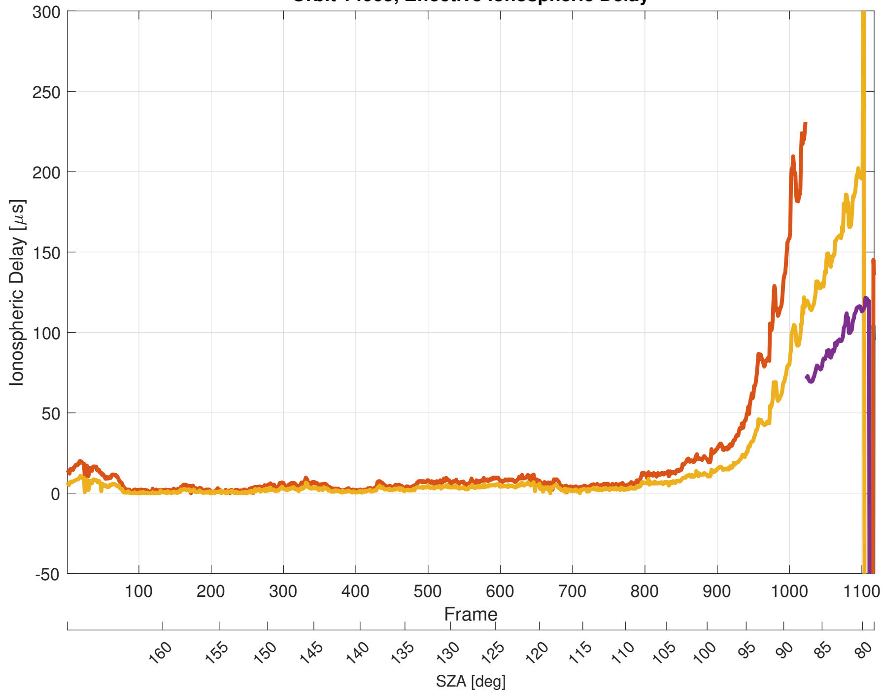
Orbit 14065, Effective Ionospheric Delay
